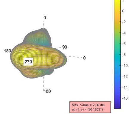
Biceps Antenna <MRG> Averaged in \phi polarization for Fat Subject
