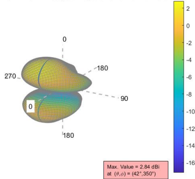
Chest Antenna <MRG> Averaged in \phi polarization for Normal Subject
