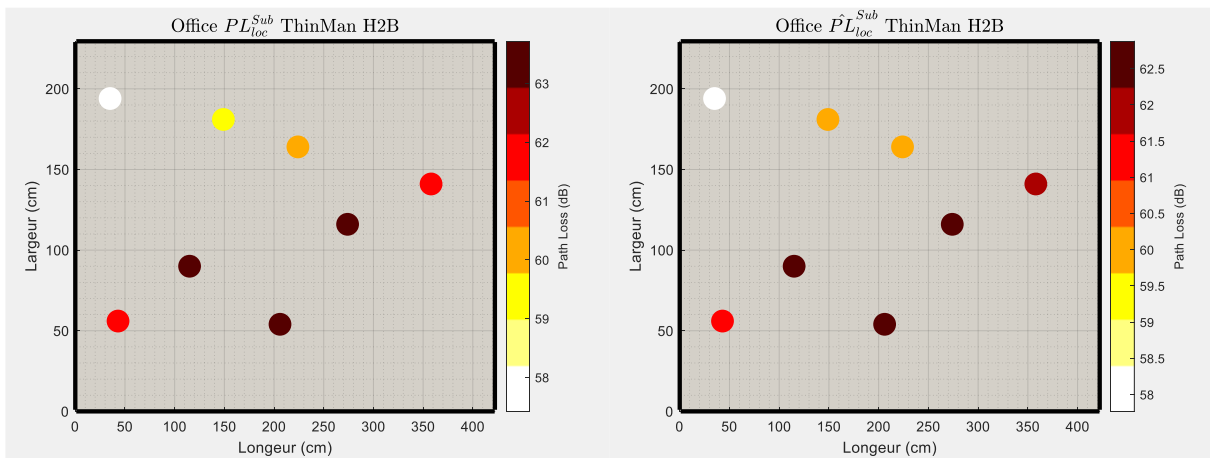
Figure_Annexe 121 PL_{loc}^{Sub} et \widehat{PL}_{loc}^{Sub} : Office, H2B.
