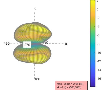
Ear Antenna <MRG> Averaged in \theta polarization for Fat Subject
