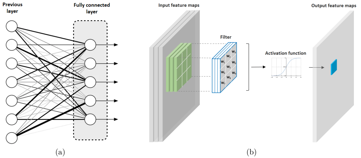
Figure 1.3 – (a) Structure of a fully connected layer: every neuron of the previous layer is connected to each neuron of the current layer (b) Structure of a convolutional layer: the input image is convolved with filters to produce feature maps.
