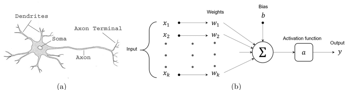
Figure 1.2 – (a) Structure of a neuron [57]: The dendrites deliver the input signals to the soma, which emits an output signal (if the input signals exceed a threshold) to the axon, which delivers it to another neuron (b) Structure of a neural network: the input signals are transformed to compute the output signal using a linear transformation, with learnable weights and biases, and a non-linear activation function.
