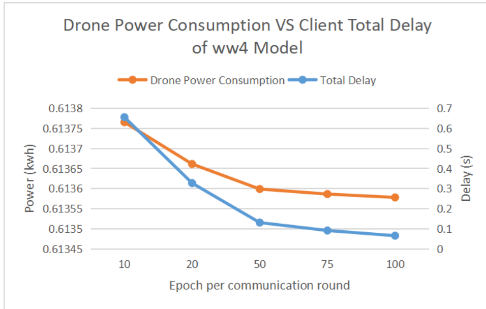
Figure 5.24: Drone power consumption and vehicle's delay
