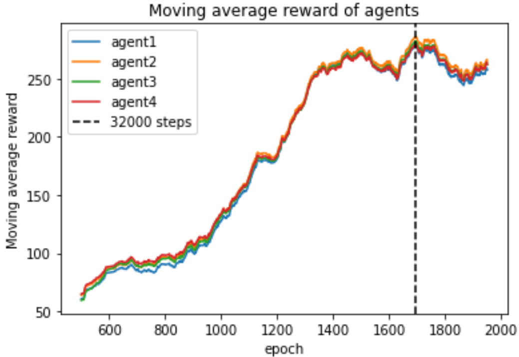
Figure 5.7: Moving average reward of agents
