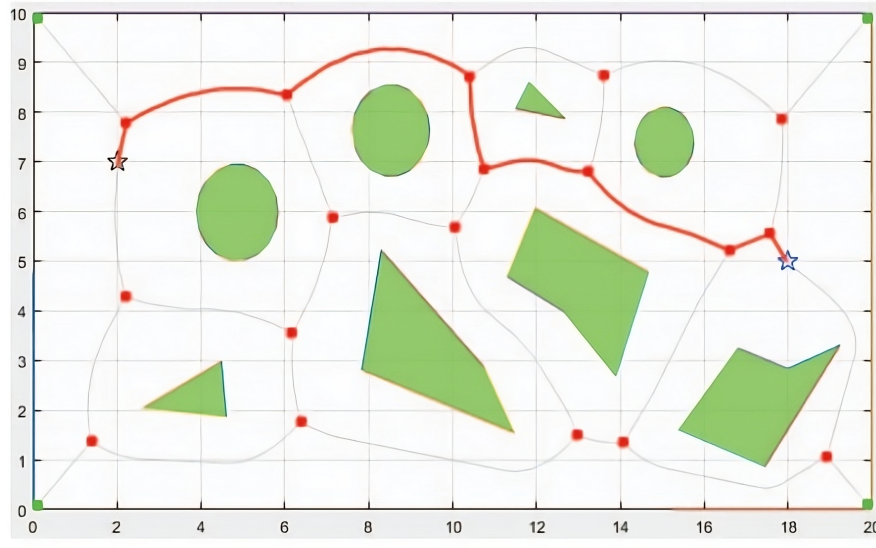
Figure 6.1: Voronoi diagram with the indicated graph branch nodes and optimal point-connected trajectory [104]
