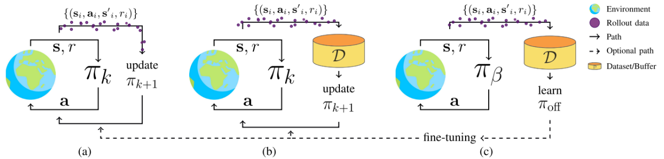
Figure 6.6: Illustration of the different RL paradigms, including (a) online RL, (b) off-policy RL, and (c) ORL. In online RL new experiences must be collected with the latest policy before making an update. In off-policy RL, we reuse previous experiences but still rely on a continuous collection of new experiences. In contrast, ORL only uses previous experiences collected with a behavior policy \pi_\beta and stored in a static dataset D to learn a policy \pi_{off} . After learning off, one can opt to fine-tune it using online or off-policy RL methods [130]
