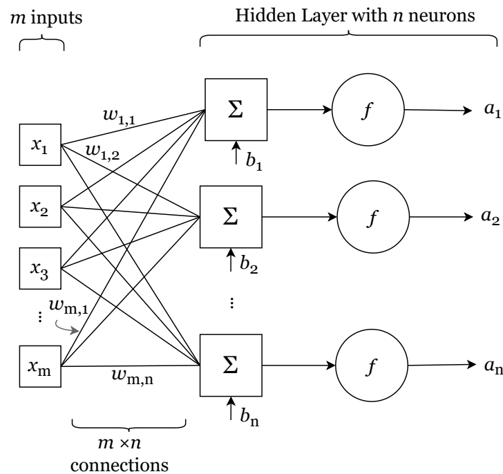
Figure 4.13: Example neural network layer with multiple neurons.
