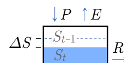
Figure 1.3: A simplified water budget showing the main water cycle components P , E , R , and \Delta S .
