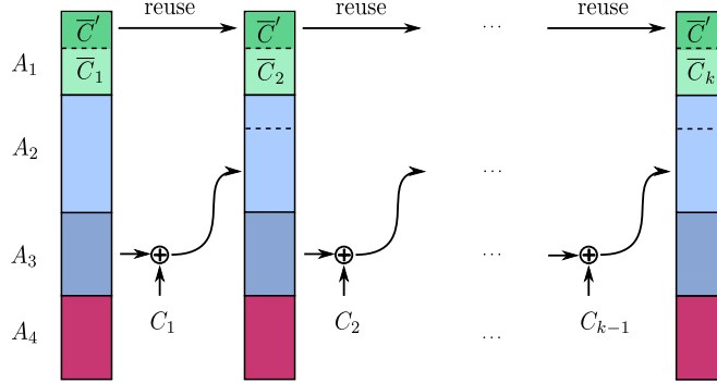
Figure 5.4: Chaining construction for block Markov encoding
