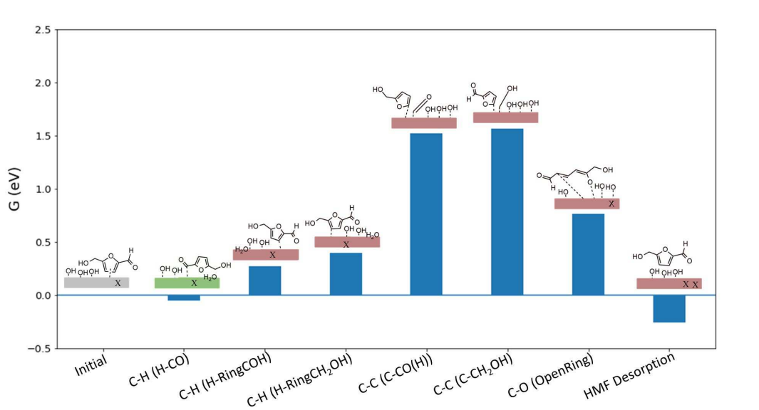
Figure 5-7 Reaction energies and scheme revealing possible degradation pathways in the transformation of HMF to the HMFC intermediates over Au catalyst at 1 bar and 110°C. Note that red is the undesired pathway, gray is the initial form before the chemical change, green is the desired pathway, X is a 1-empty catalyst slab, and all bonded species that have a dashed line or are placed on the slab. All surface species are singly mono-adsorbed (not co-adsorbed) on a slab.
