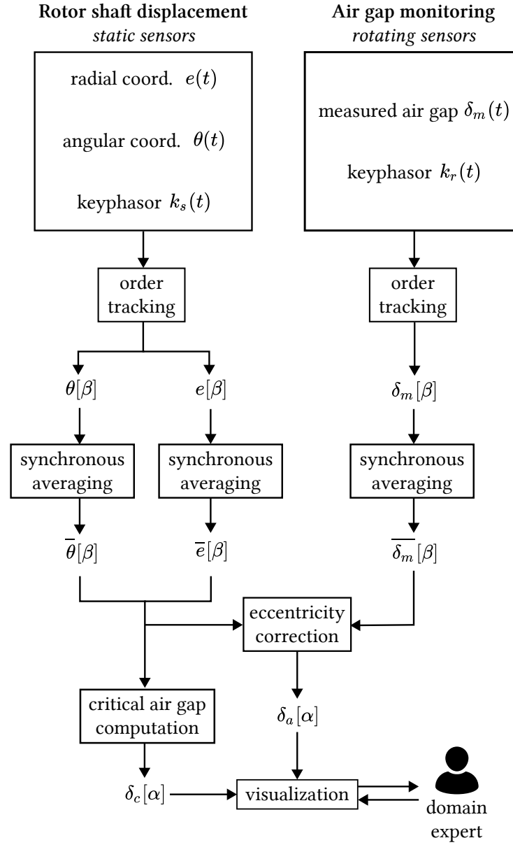
Figure 7.11 – Schematic of the proposed data science pipeline.
