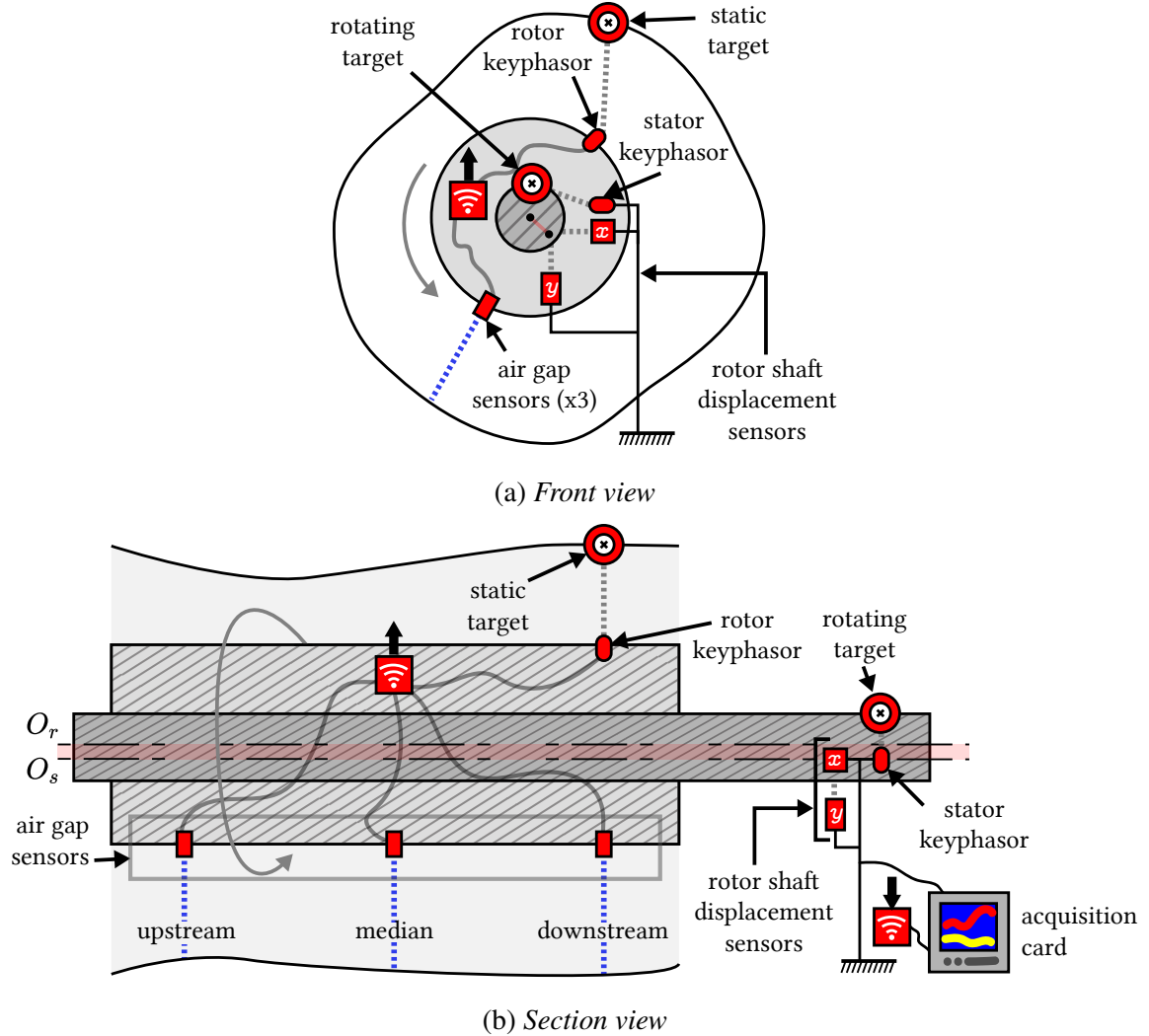
Figure 7.4 – Schematic of the turbine instrumentation.
