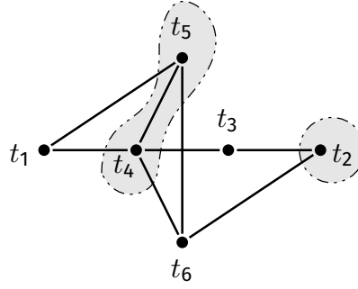
Figure 3.3 – Conflict-graph CG_{\Phi}(\phi_f, r_{toy}) . An MVC is encircled.
