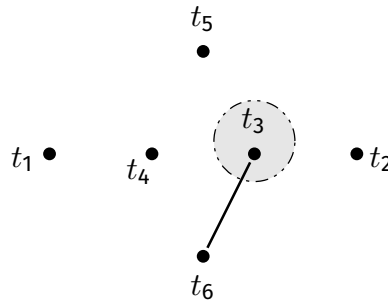
Figure 3.2 – Conflict-graph CG(\phi_f, r_{toy}) . An MVC is encircled.
