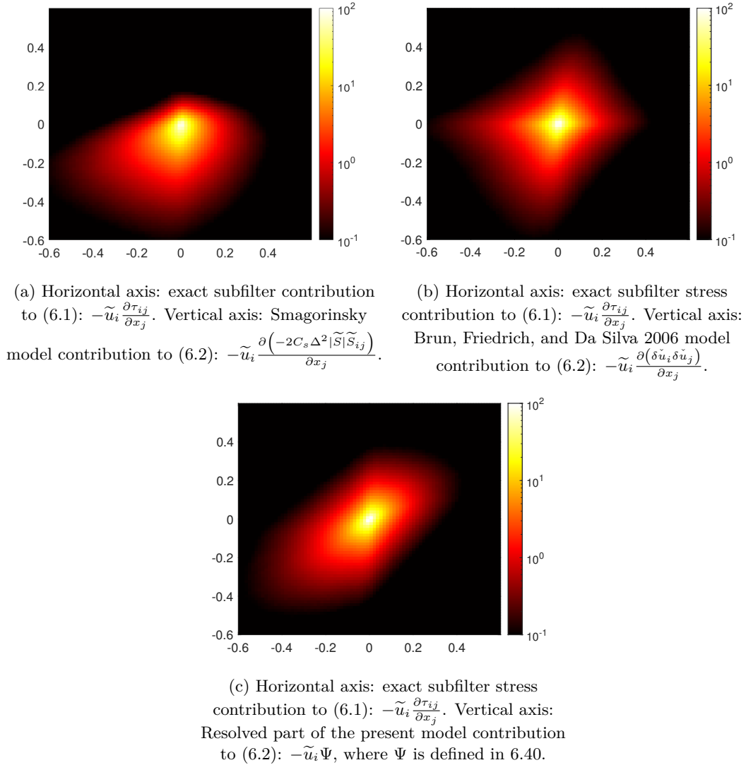
Figure 6.8: Joint PDFs of modelled subfilter stress contributions to (6.2): -\tilde{u}_i \widehat{\frac{\partial \tau_{ij}}{\partial x_j}} with exact subfilter stress energy contribution to (6.1): -\tilde{u}_i \frac{\partial \tau_{ij}}{\partial x_j} evaluated in the Taylor-Green DNS simulation with \Delta \approx 8\eta and with scaling coefficient.
