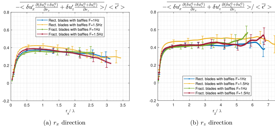
Figure 4.11: Interscale transfer rate estimate
