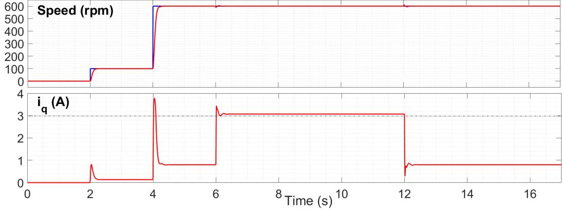
Figure 4.27: Simulation results of the motor speed and q-axis ( i_q ) current using flatness-based controller with traditional trajectory planning under significant change of load torque ( T_L ).
