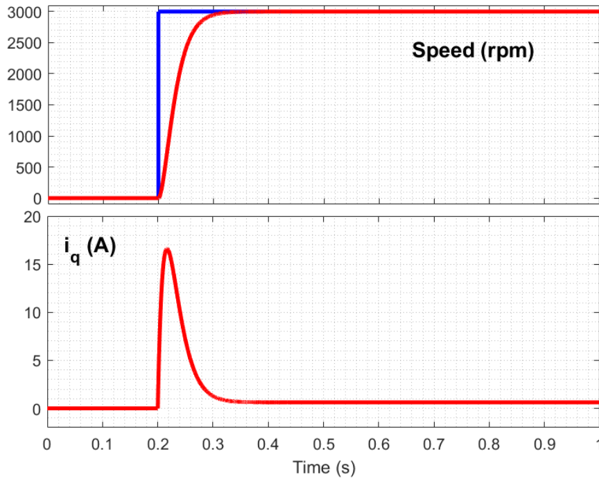
Figure 4.16: Simulation results of input ( y_{\Omega,inf} ) and output ( y_{\Omega,ref} ) of the conventional trajectory planning with \omega_f = 60 rad/s, resulting in significant current overshoot.
