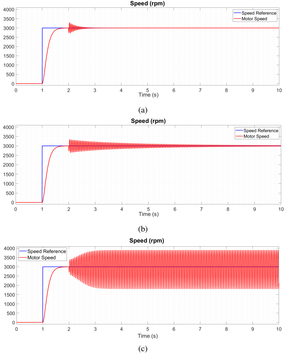
Figure 4.9: Simulation results of motor speed with flatness-based control method (a) when L_d = L_q = 5 L_{nom} . (b) when L_d = L_q = 5.5 L_{nom} . (c) when L_d = L_q = 6 L_{nom} .
