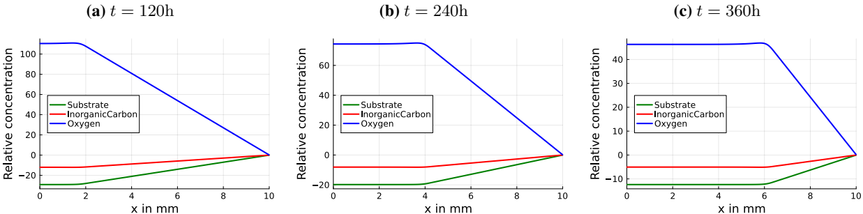
Figure 6.9: Solutes relative concentration for different times
