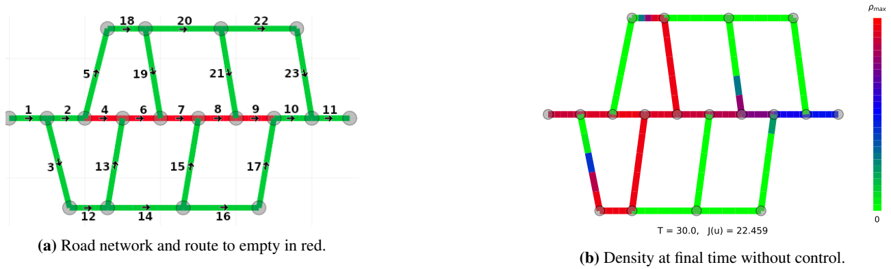
Figure 2.6: (Three lanes network) Left: Three lanes network configuration. Road 1 is incoming and road 11 is outgoing and all the others are directed from left to right. The route to empty (4, 6, 7, 8, 9) is in red. Right: Numerical simulations without control at time T = 30 .
