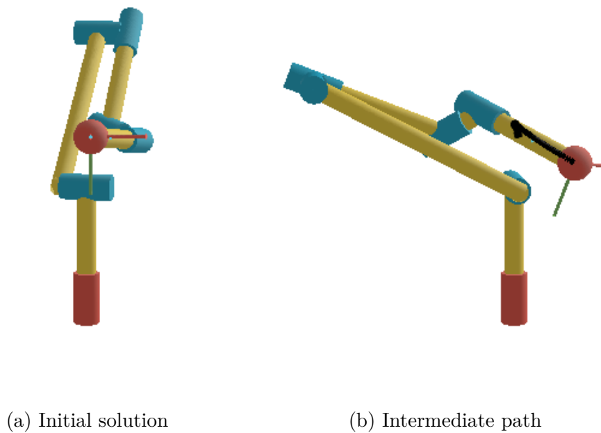
Figure 4.11 – Nonsingular change of solutions: IKS VII \rightarrow VIII.
