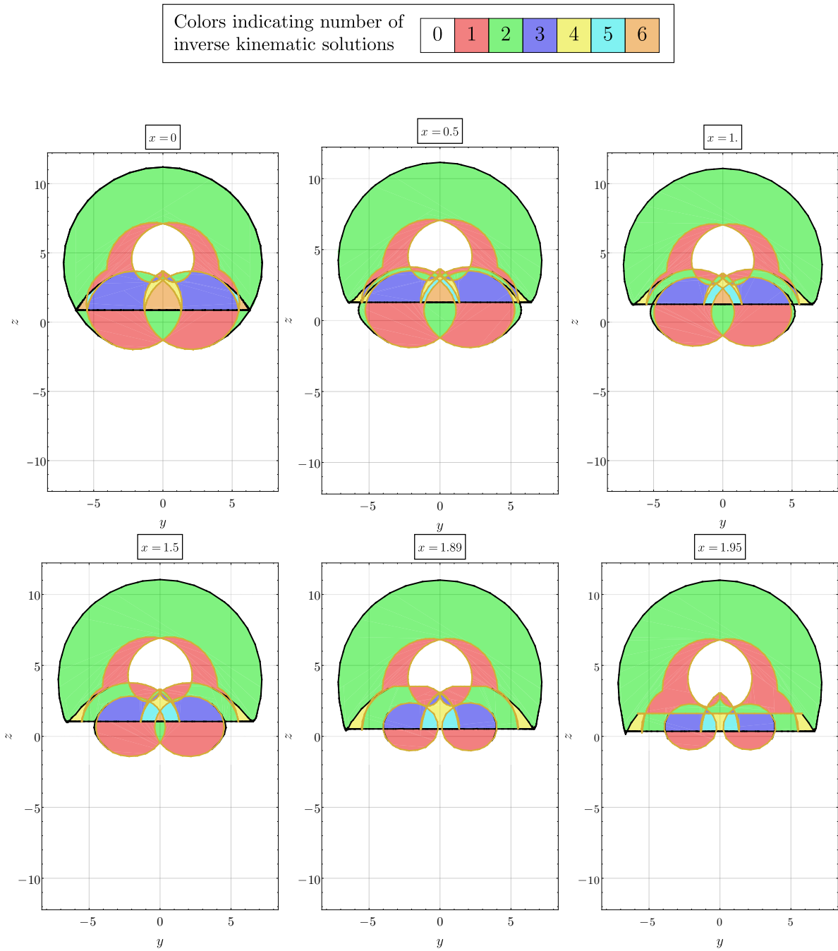
Figure 7.22 – Sections of the workspace at x \in [0, 1.95] for the manipulator b = 1, l = 2, a = 2 .
