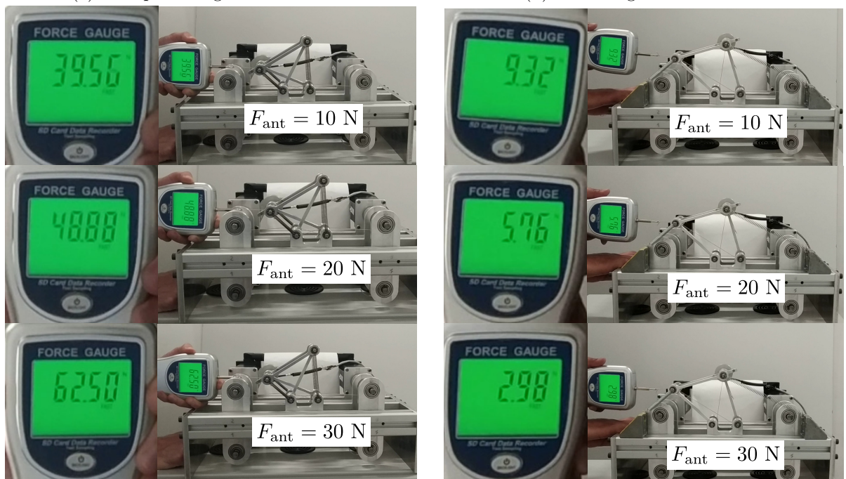
(c) Mechanism with crossed limbs
