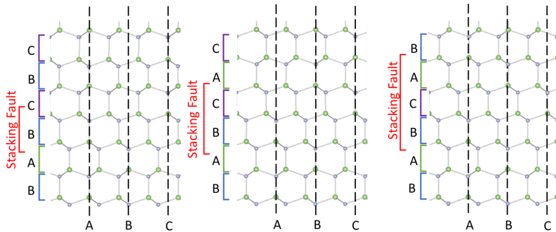
Figure I-7: I1 (a), I2 (b) and E (c) configuration for basal stacking faults.
