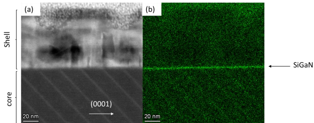
Figure III-12: (a) ADF and (b) Si-EDX mapping of a nanowire at the junction between the core and the shell (Longitudinal lamella, sample A)
