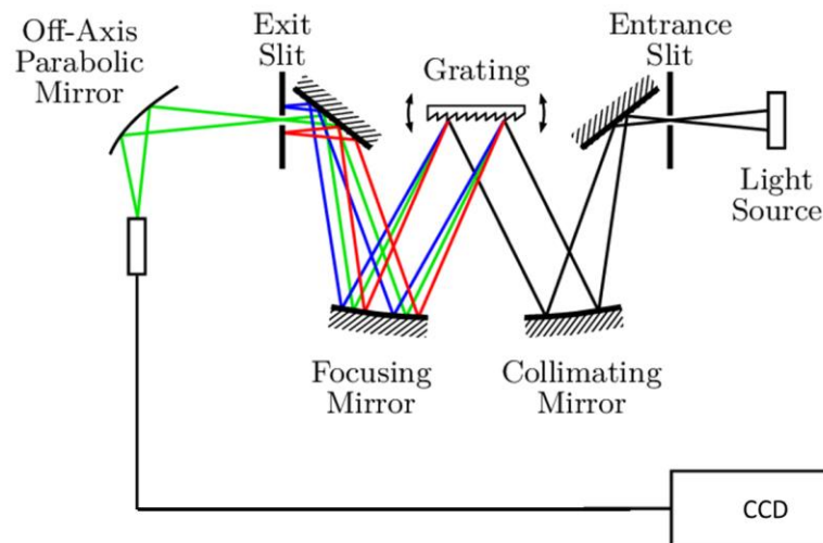
Figure II-11: Scheme of a monochromator/CCD setup used to measure spectra in PL (adapted from ref 4 )
