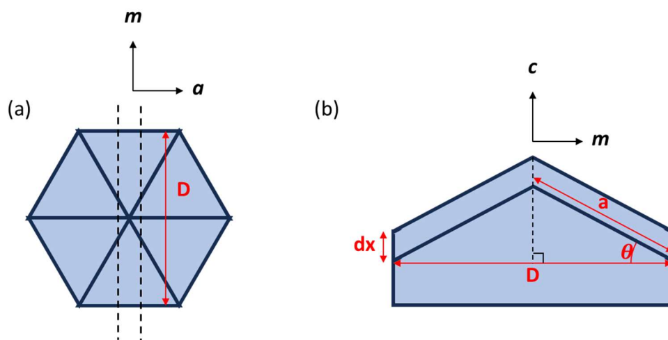
Figure D-1: Geometrical parameters of the Si-rich markers in transversal (a) and longitudinal (b) view
