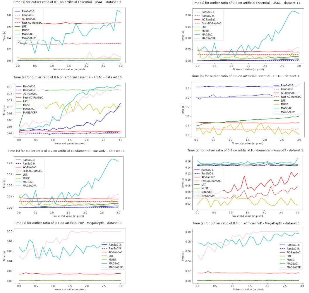
Figure 3.1: Runtimes over different inlier noise levels and outlier ratios. The fitting problem, dataset name, and image pair number are in each graph title. Ransac- \sigma corresponds to RanSaC with user threshold \sigma .
