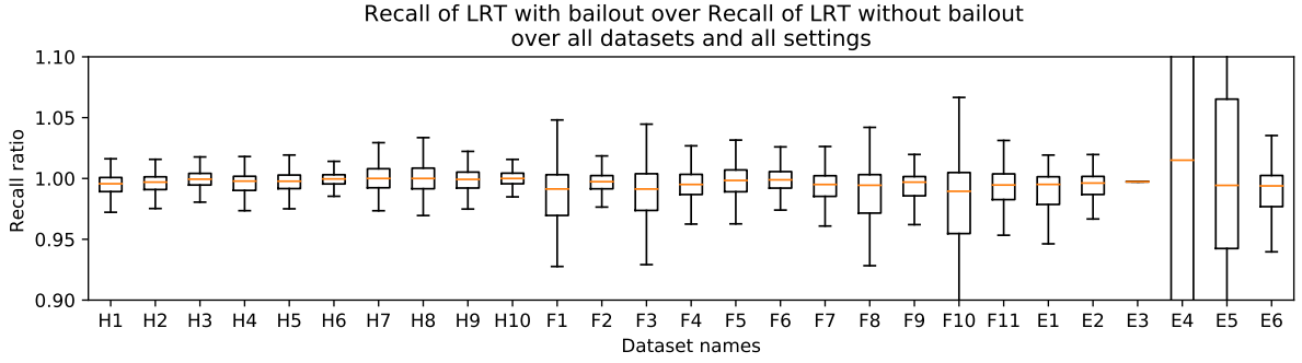
Figure 3.7: Boxplot of the ratio of the recall of LRT with the early bailout strategy and without the bailout. Results are presented across all available USAC [73] datasets and over a high range of semi-artificial dataset settings. H stands for homography estimation, F for fundamental matrix estimation and E for essential matrix estimation with same numbering as USAC. Dataset E4 and E4 are cut as they spread much more than others and made them hard to read. For E4 the quartiles are [0.89, 1.15] and the whiskers are [0.51, 1.56] . For E5 the quartiles are [0.94, 1.07] and the whiskers are [0.78, 1.25] .
