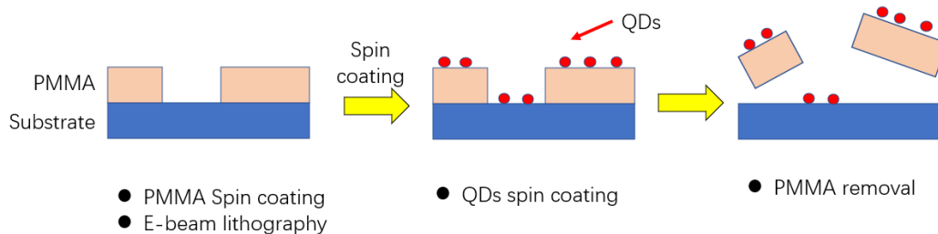
Figure 3.26: Procedures of depositing QD on the substrate.
