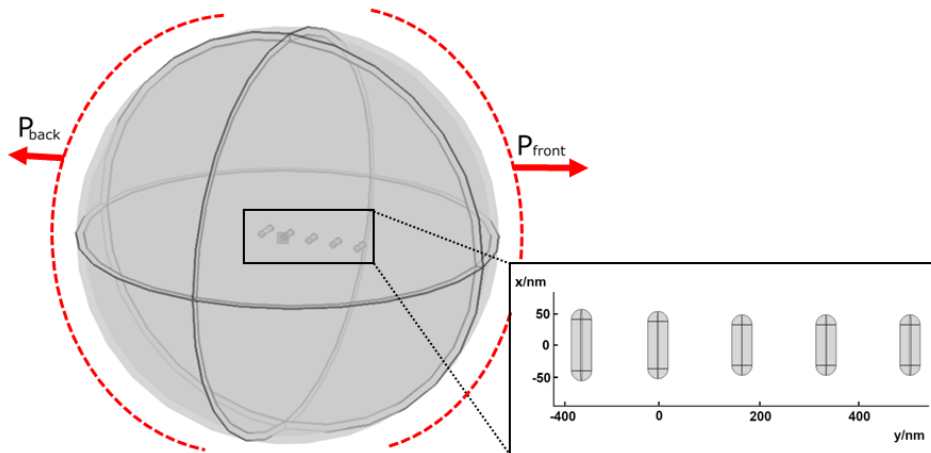
Figure 3.3: Model of simulation domain in free space. Red arrows represent integration surface of far-field power.
