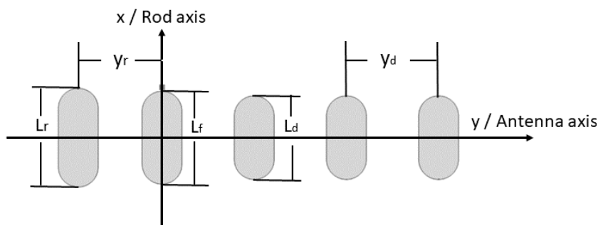
Figure 3.1: Scheme of Yagi-Uda antenna.
