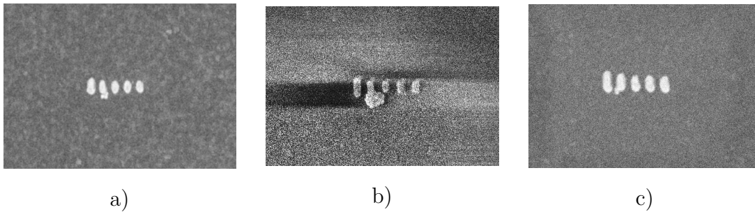
Figure 3.42: SEM images of quantum dots deposited to Yagi-Uda antenna a) 60 nm hole, b) 100 nm hole before optimization, c) quantum dots slightly off-deposited.
