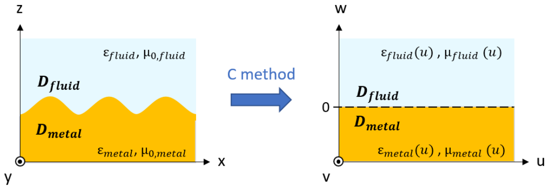
Figure 3.15: Sketch of the transformation of a corrugated grating into a flat interface by the C method.
