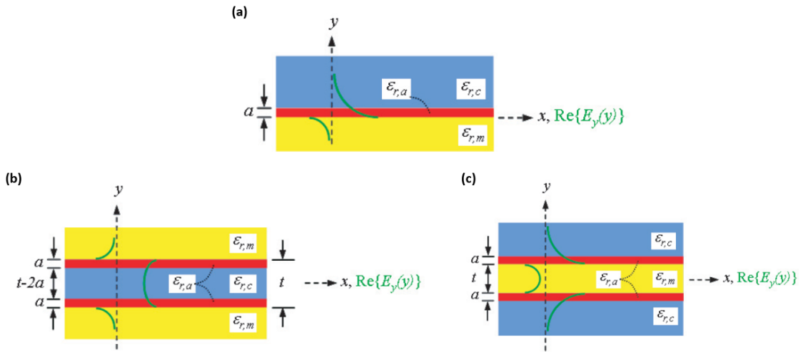
Figure 2.12: Sketches of 1D surface plasmon waveguide structures based on (a) a single interface metal-dielectric waveguide, (b) a MIM waveguide, and (c) a IMI waveguide. The metal layers with a relative permittivity \epsilon_{r,m} are represented in yellow, and the dielectric media with a relative permittivity \epsilon_{r,c} in blue. The dielectric adlayers with a thickness a and a relative permittivity \epsilon_{r,a} are coloured in red. The real part of the main transverse electric field component ( \text{Re}\{E_y\} ) of the mode of interest is sketched in green on all structures. These figures are extracted from the article [101]. Reprinted with permission from IOP Journal, doi:10.1088/1367-2630/10/10/105010. Copyright 2015 The Authors, licensed under a Creative Commons Attribution (CC BY) license.
