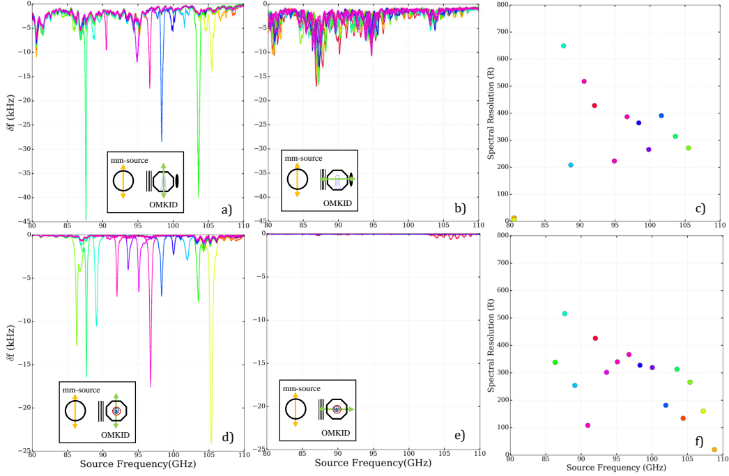
Figure 7.6: The spectral response and the resolution of OM-D4, illuminated with the mm wave source through four eccosorbs attenuated layers. The top panels of (a), (b) and (c) show the results for direct illumination. The panel below i.e., (d), (e), (f) shows the measurement when the incoming signal is guided through horn and waveguide transition on the slot antenna. Different colours refer to different channels.
