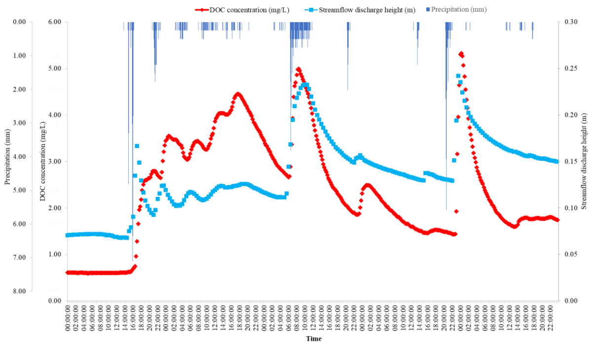
Figure 8.15: Correlations between rainfall, streamflow discharge and DOC probe concentrations during a rainfall event from the 6th of February to the 10th of February 2020 for CP-VI and CP-IX
