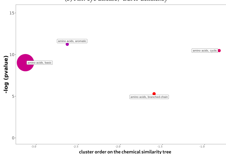
Figure 35: ChemRich using sampling predictions for the 54 metabolites from Thiele et al. for three IEM conditions.
