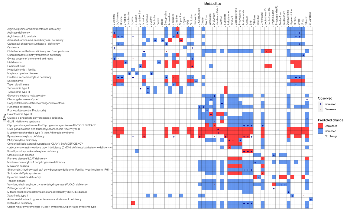
Figure 21: Reproduction of Thiele et al. 's heatmap using Python. Blue and red tiles represent biomarkers that are predicted to be increased or reduced, respectively. Table entries marked with '+' or '-' represent elevation or reduction in the metabolite's concentration in biofluids according to the gold standard [131], respectively.
