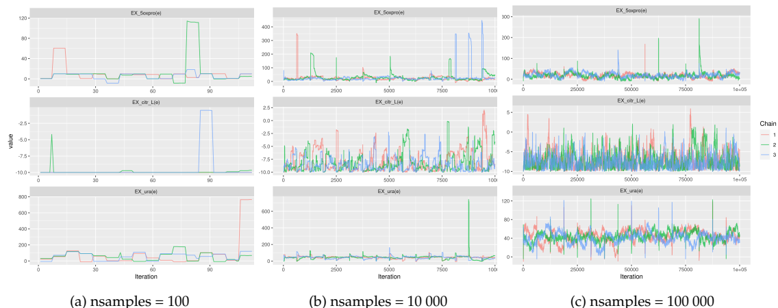
Figure 40: Trace plots for 3 random exchange reaction fluxes using (a) 100, (b) 10 000 and (c) 100 000 samples, with 3 independent runs for each. The x-axis shows the iterations along the sampling process while the y-axis shows the flux value for each iteration. The three colours are the three independent runs. The rows in each subplot represent the same randomly picked exchange reactions.
