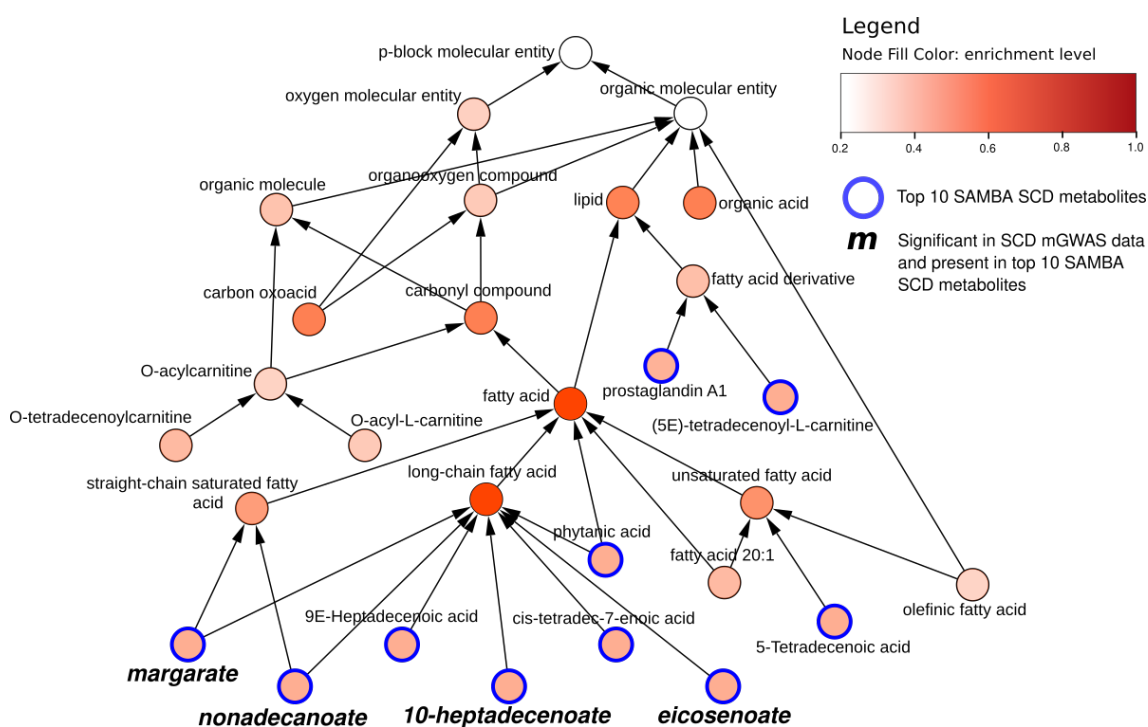
Figure 32: Hierarchical ChEBI graph of the top 10 metabolites predicted to be differentially abundant (outlined in blue) by SAMBA for SCD, extracted using BiNChE. The node colour corresponds to the BiNChE enrichment level. The metabolites in bold & italic were significant in the mGWAS dataset for SCD.
