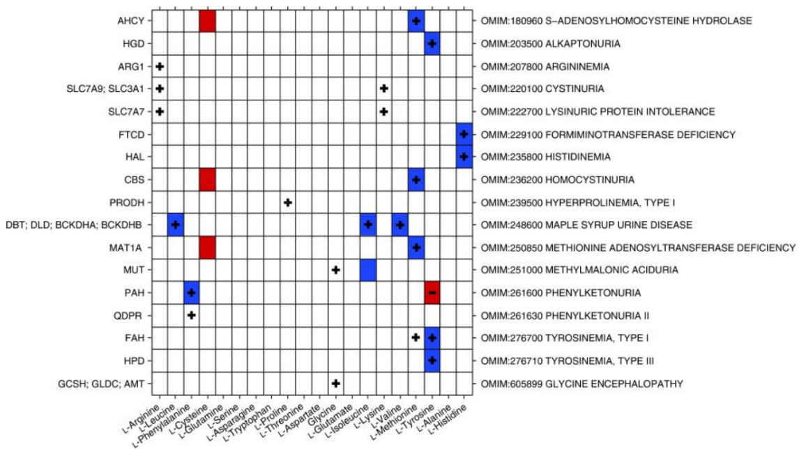
Figure 18: Prediction of amino acid biomarkers for a set of amino acid metabolic disorders from Shlomi et al. Rows represent metabolic disorders and columns represent amino acids. The causative gene's name is indicated on the left. Blue and red entries represent biomarkers that are predicted by our method to be elevated or reduced, respectively. Table entries marked in '+' or '-' represent elevation or reduction in the metabolite's concentration in biofluids according to OMIM, respectively.
