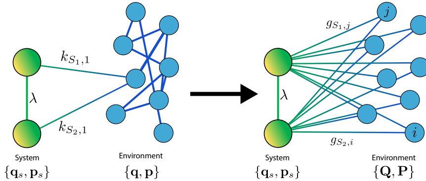
Figure 8.2: Interaction between the system and the environment. Left: the system interacts with the environment (in the coupled picture \hat{\mathbf{q}}, \hat{\mathbf{p}} ) with couplings k_{S_i,1} and k_{S_2,1} in a minimal coupling scenario. Right: This system-environment network can be equivalently described in the picture where the oscillators of the environment are uncoupled (quadratures \hat{\mathbf{Q}}, \hat{\mathbf{P}} ), where the interaction among the system oscillators and the uncoupled environment oscillators is described by the vector \mathbf{g}_{S_i}^T .
