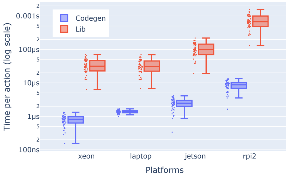
Figure A.2: Average time per TPG inference with the generated code and with the library. Each box-plot represents the statistics for the 50 TPG (5 games×10 TPG) run on a platform.
