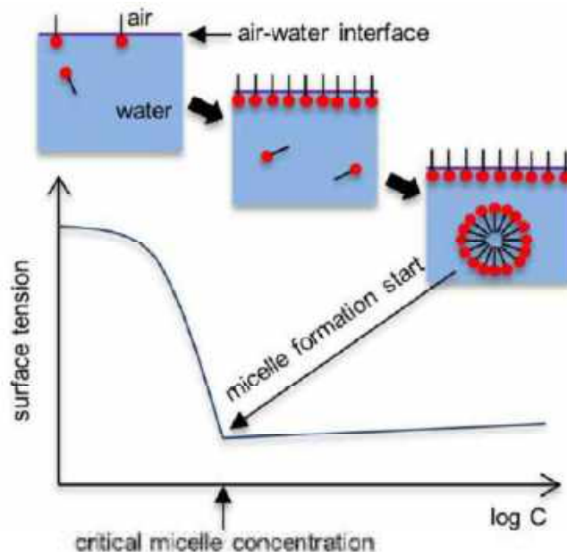
Figure 1.12. Schematic of the change in surface tension observed during micelle formation. Reproduced from 53 .
