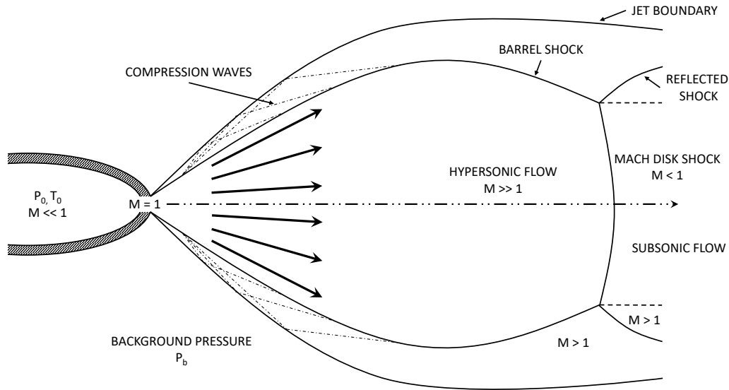
Figure 4.4 : Schematic of an extremely underexpanded free jet expansion (inspired by ROWE & CANOSA (2022)).
