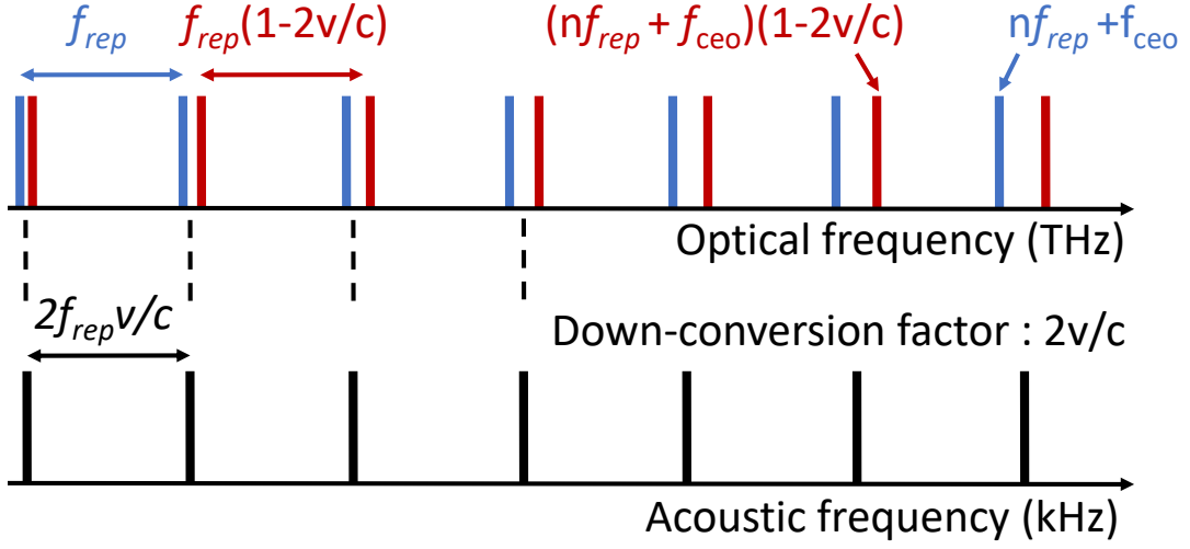
Figure 1.12 : Down-conversion of a frequency comb from optical to acoustic frequencies by a Fourier transform spectrometer. The beatnotes from pairs of fixed (blue) and Doppler-shifted comb modes (red) on the photodetector yield an acoustic comb with a mode spacing 2f_{rep}v/c . The down-conversion factor is 2v/c with v the speed of the interferometer translation stage and c the celerity of light.
