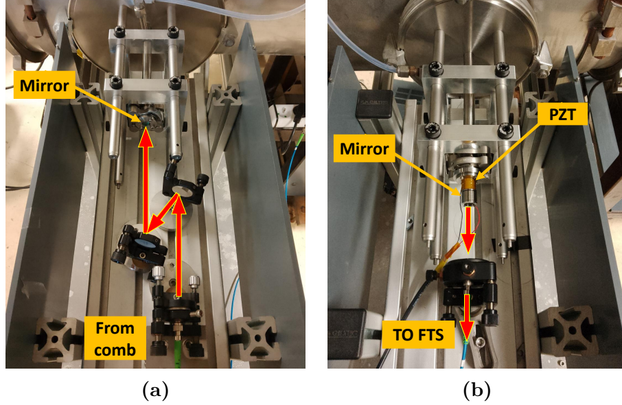
Figure 4.9 : Pictures showing the mirror mounts and cages mounted on the jet cell flanges. The red arrows indicates the path of the comb light. (a) - Input mirror cage with comb light coupled to free space from fiber and injections mirrors. (b) - Output mirror cage (PZT visible, mounted on the mirror) with collimator and fiber going to the FTS.
