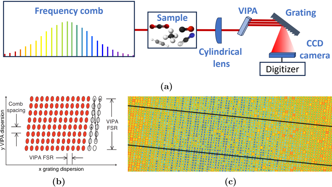
Figure 1.9 : (a) - Schematic of a VIPA spectrometer. The comb light is focused as a plane with a cylindrical lens in the VIPA aperture. The VIPA diffracted beams are then cross-dispersed with a grating, and imaged onto a CCD camera. (b) - Schematic of the output of a VIPA spectrometer recorded onto a camera. The resolved comb modes (red dots) are separated by the comb mode spacing along the y axis and by the VIPA FSR along the x axis. The full y range corresponds to one VIPA FSR. The frequency axis is shown on the right part of the image, with black arrows on white dots. (c) - Image from a camera. Each dot correspond to a resolved comb modes. The different colors correspond to different intensities of the comb modes, the darker the more optical power. Some brighter spots are visible, due to molecular absorption of certain comb modes. (b) and (c) reproduced from DIDDAMS et al. (2007).
