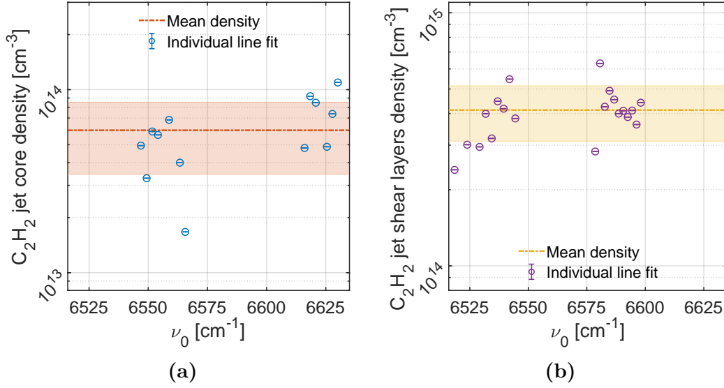
Figure 4.21 : (a) - C_2H_2 density in the isentropic core (blue circles) obtained after independently fitting each line, with the corresponding statistical uncertainty from the fit as the errorbar. The density is shown on the y axis with a log scale. Dotted red trace: mean value. Shaded red region: standard deviation. (b) - C_2H_2 density in the shear layers (purple circles) with the corresponding statistical uncertainty from the fit as the errorbar. Dotted yellow trace: mean value. Shaded yellow region: standard deviation.
