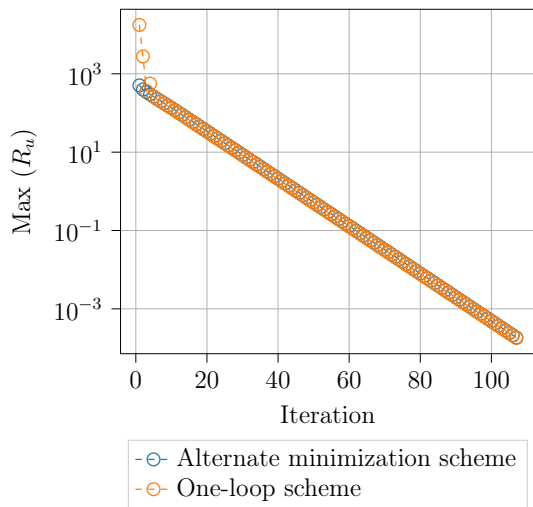
(a) Convergence of the residual at A.
