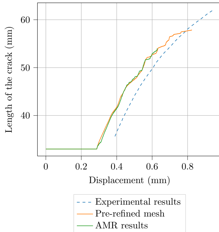
(b) Crack propagation with the fitted model
