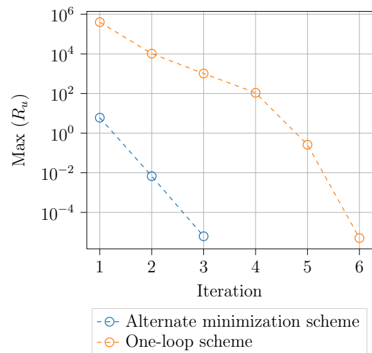
(b) Convergence of the residual at B.
