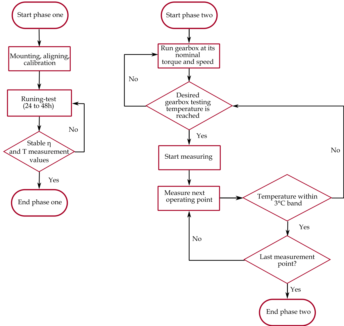
Fig. 127: Measurement procedure
