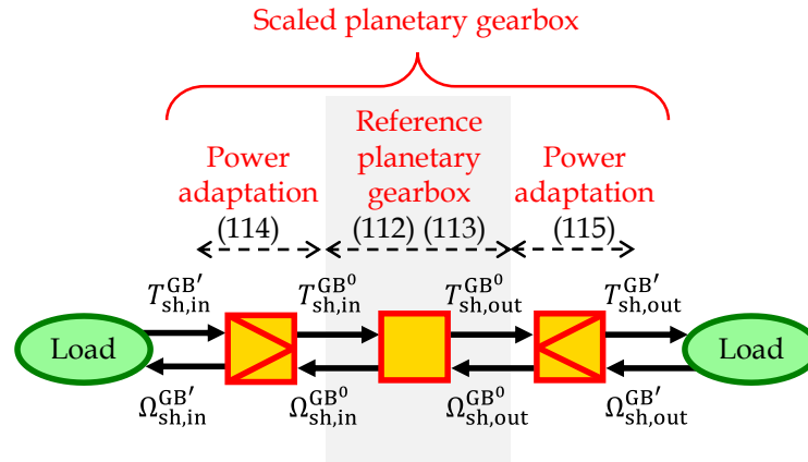
Fig. 76: EMR-bases scaling laws of planetary gearboxes
