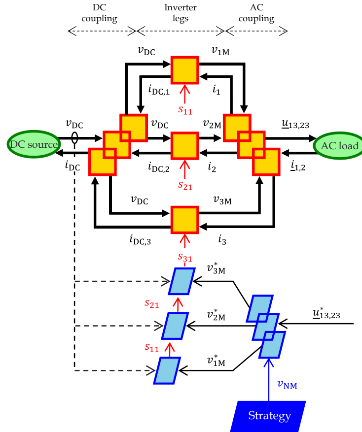
Fig. 141: EMR of a voltage-source inverter
