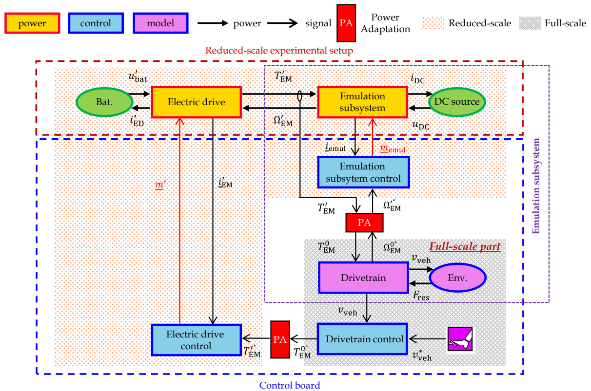
Fig. 114: Organization of reduced-scale hardware-in-the-loop testing. Variables denoted with an apostrophe ' refer to scaled parameters, while the superscript 0 represents the corresponding full-scale parameters.
