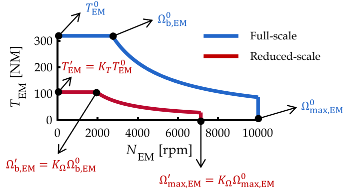
Fig. 115: Impact of the scaling factors on the torque-speed envelope of the electric drive system
