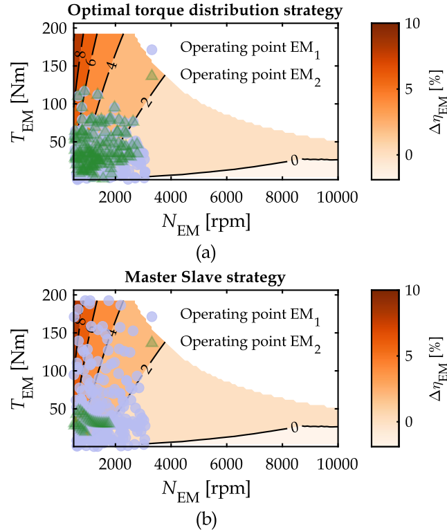
Fig. 149: Comparison of the operating points resulting from the torque distribution strategies for the NYCC driving cycle. The results are visualized in a contour map that shows the difference in terms of efficiency \Delta \eta_{EM} between linear scaling and geometric scaling methods of electric machines. Note that one contour map is used as the machine used for the MCM topology is identical.
