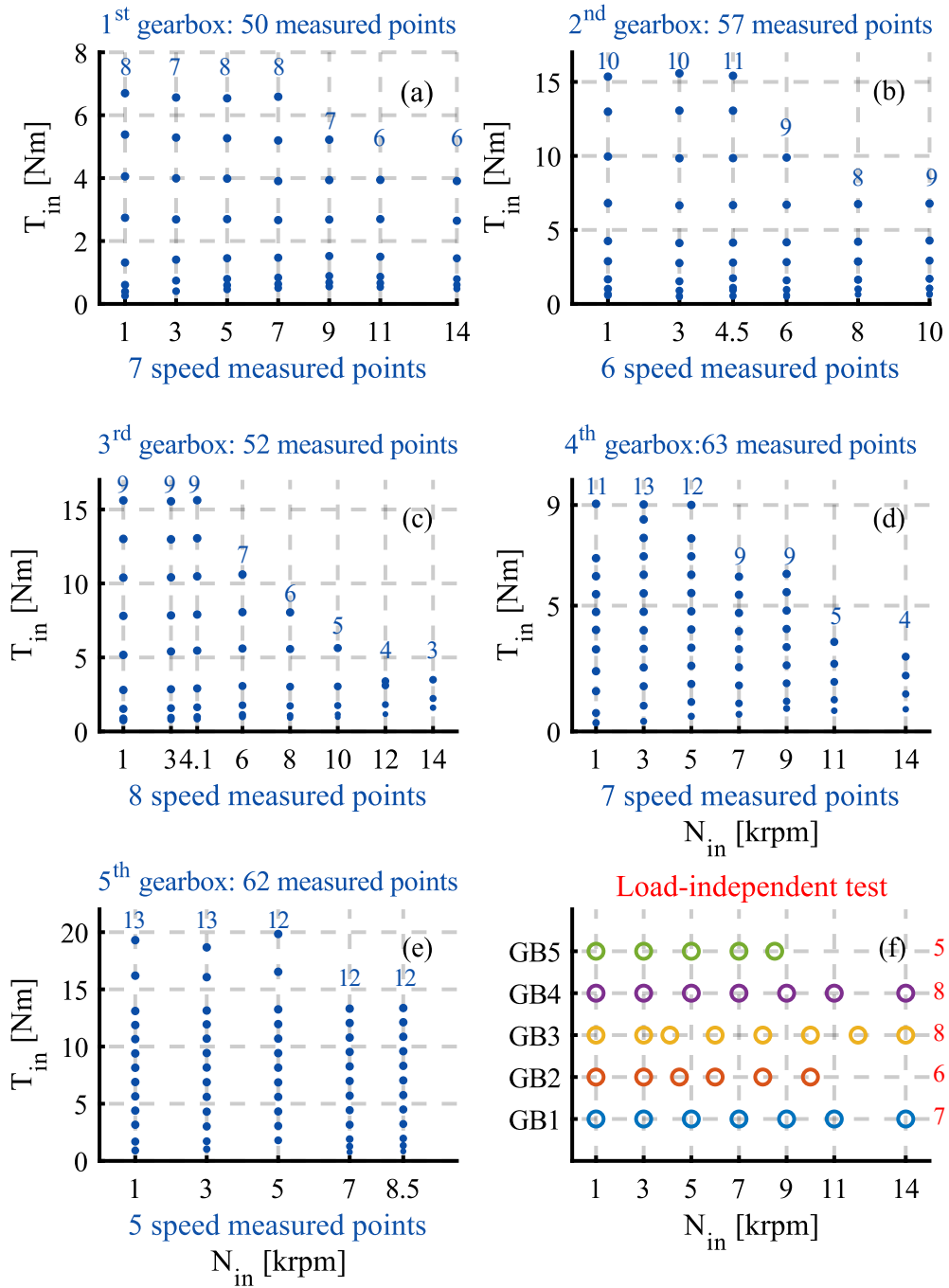
Fig. 128: An overview of the tested points for each gearbox during loaded (a)-(e) and unloaded tests (f). At the top of each subfigure (a)-(e), the total number of measured points of loaded tests is indicated. The number of measured torque points is specified for each measured speed. Lastly, the abbreviation "GB" in (f) refers to the term "gearbox".
