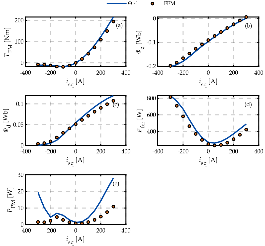
Fig. 36: Validation of the upscaling case considering the choice \theta \sim 1 for a current i_{sd} = 0
