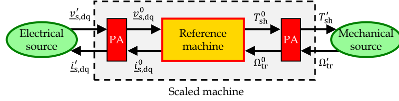
Fig. 42: Proposed structural methodology of the scaled machine
