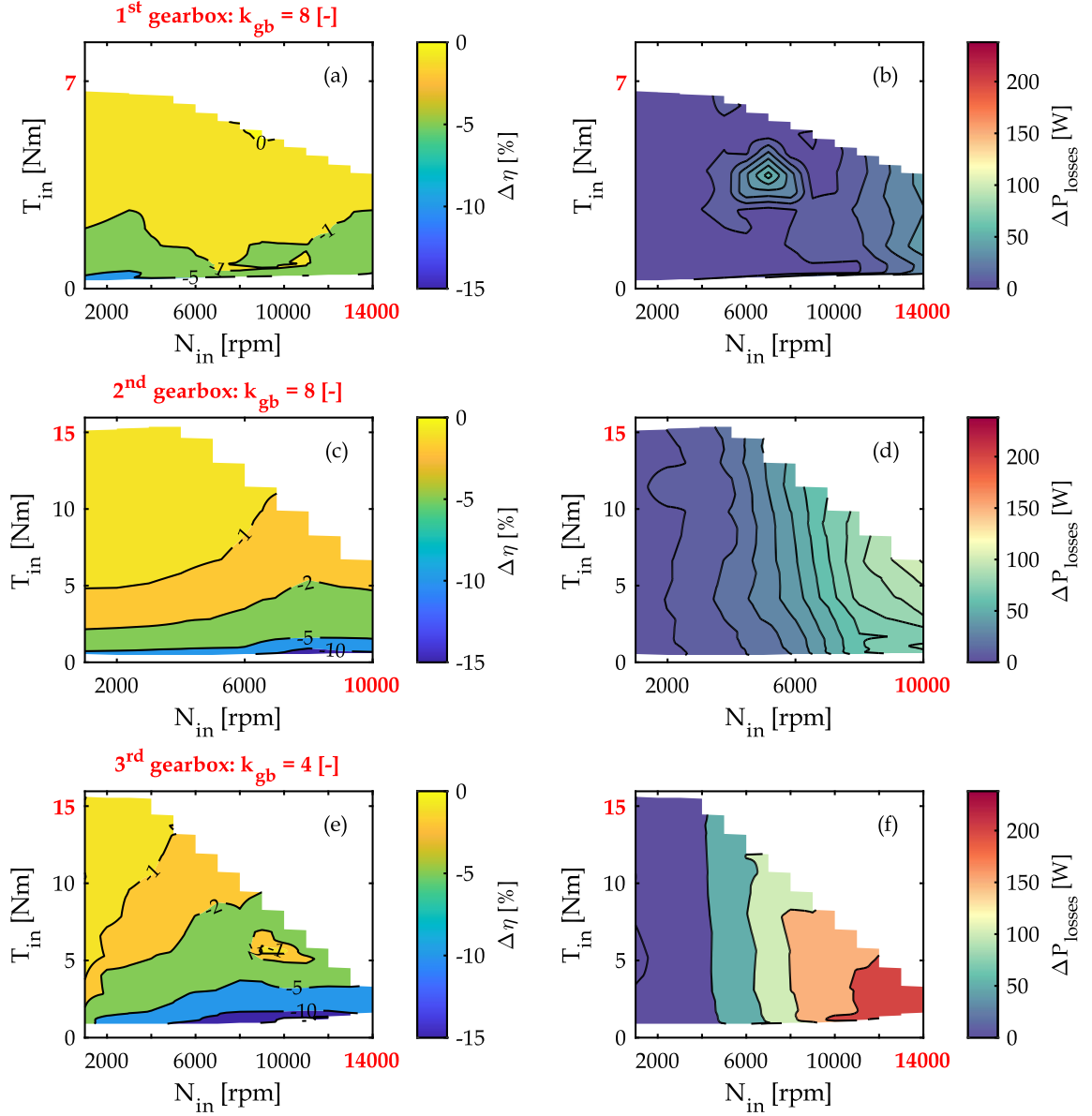
Fig. 135: Comparison between efficiency and loss results between temperatures of 30°C and 70°C. The results from the test using 50°C are considered as a reference. Negative values of the difference in terms of efficiency mean that the test using 50°C resulted in lower efficiency results. Each row in the figure corresponds to a specific gearbox.
