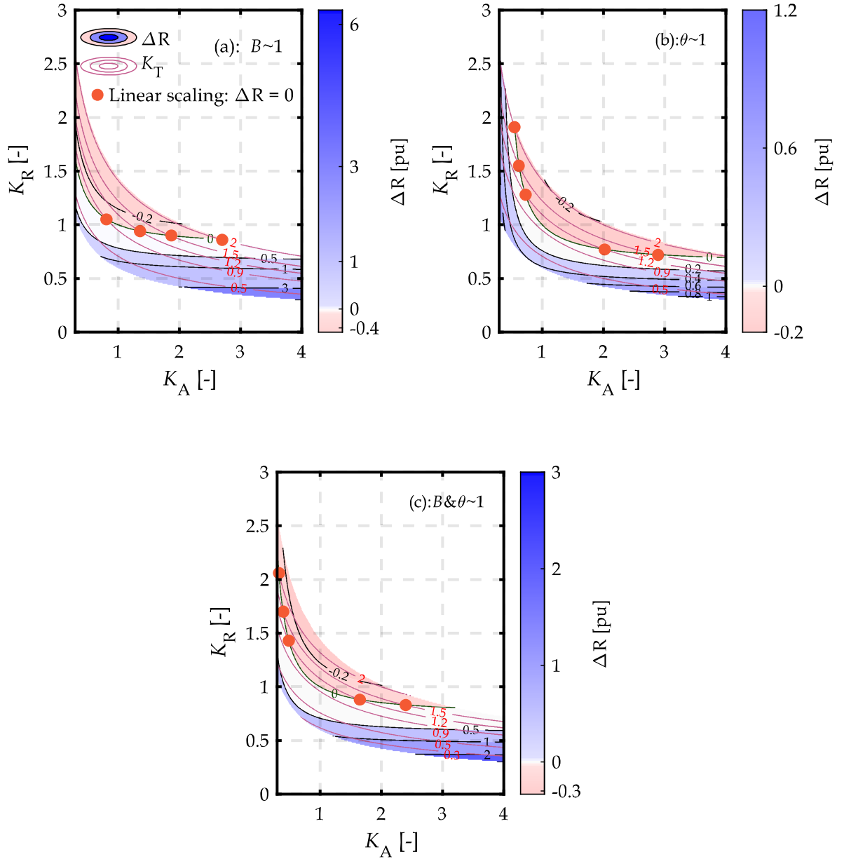
Fig. 123: Equivalent resistance term \Delta R (black contour lines) in per-unit and torque scaling factor K_T [-] (purple contour lines) as a function of axial K_A and radial K_R scaling factors.
