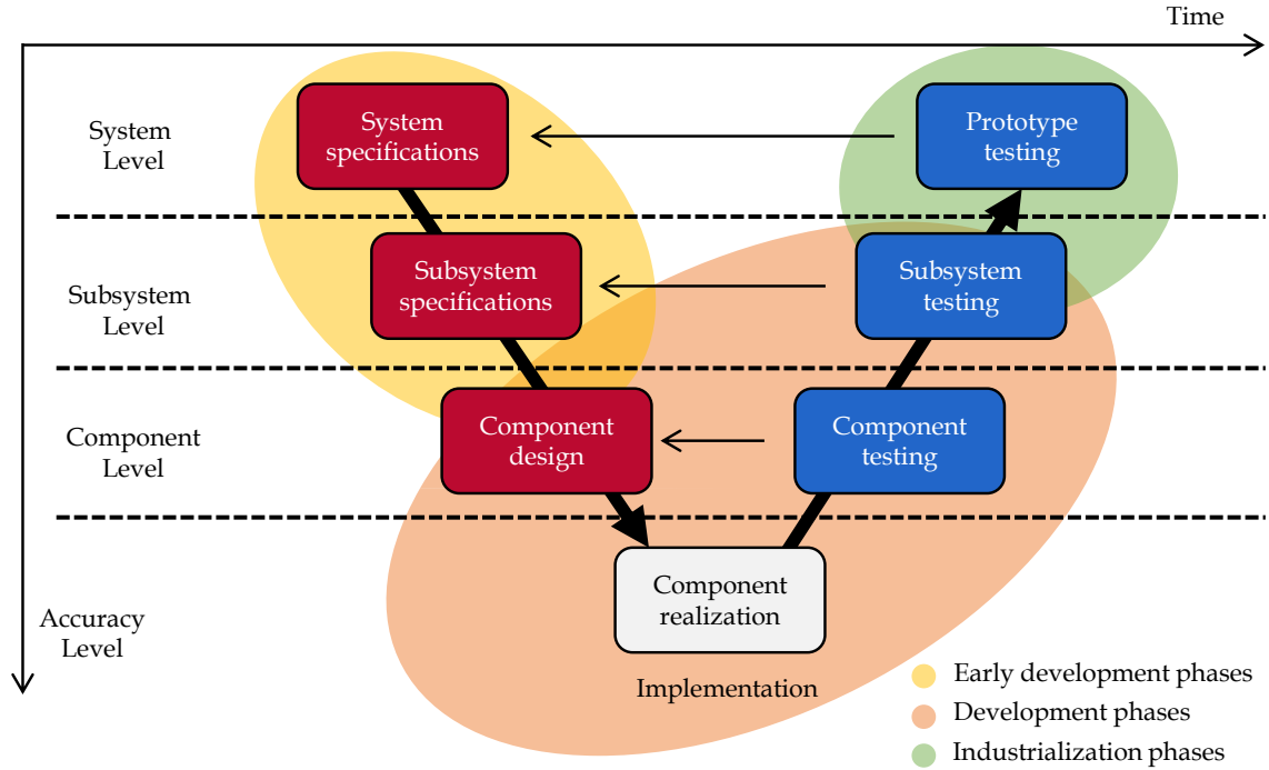
Fig. 8: V-model for industrial product development
