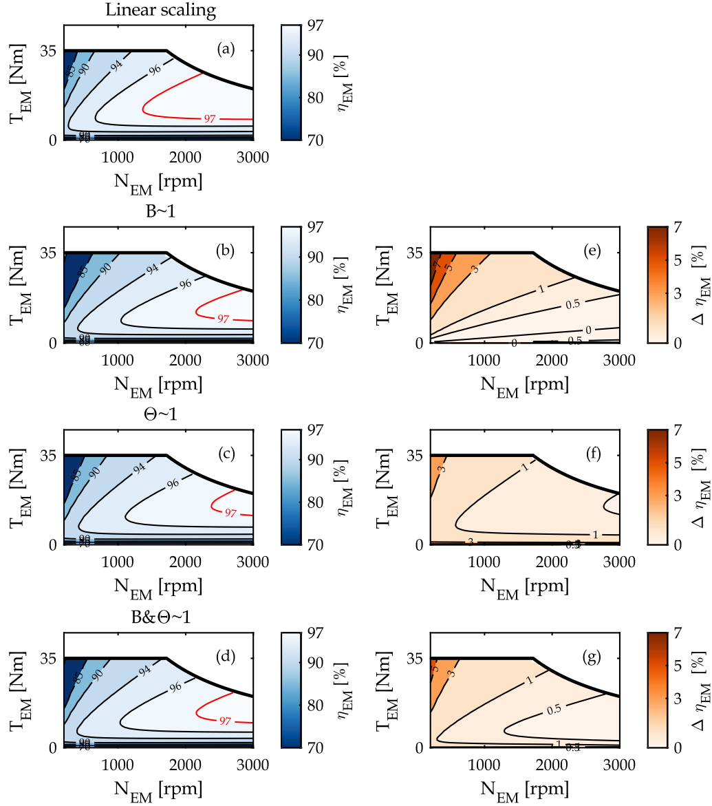
Fig. 122: Efficiency maps \eta_{EM} in [%] in the torque-speed plane using linear and geometric scaling laws for an upscaling case with a torque scaling factor of 0.5. The second column figures represent the efficiency difference \Delta \eta in [%] between linear and each choice of geometric scaling laws. Positive values for \Delta \eta mean that linear scaling overestimates the efficiency as compared to geometric scaling and vice versa.
