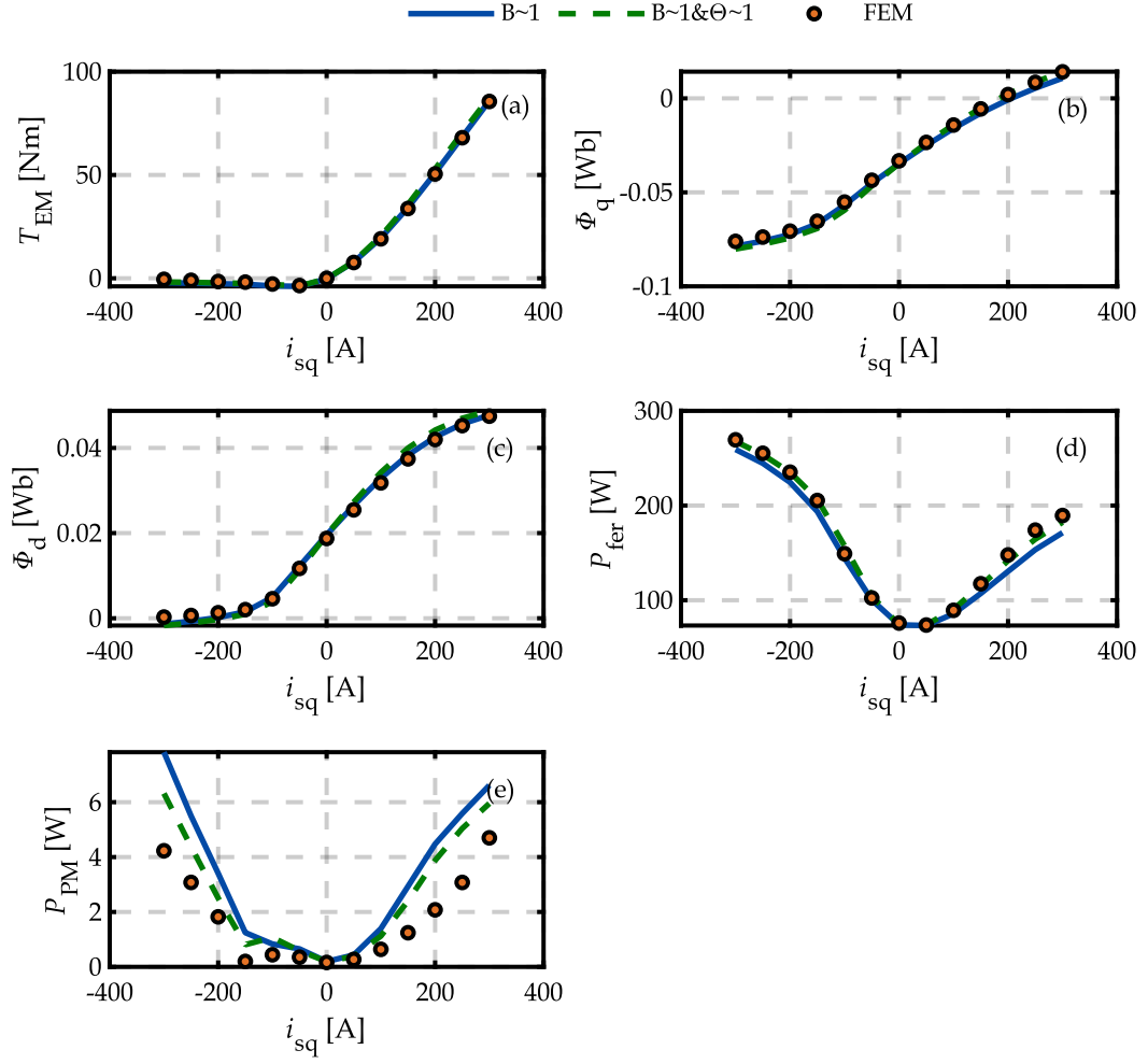
Fig. 37: Validation of the downscaling case considering the choice B \sim 1 , and B \sim \Theta \sim 1 for a current i_{sd} = 0
