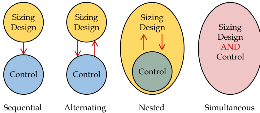
Fig. 16: Optimization framework for system-level design of the electric-axle
