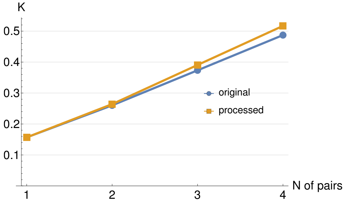
Fig. 6.4 Key rate before and after crosstalk processing. For this optimization, the limited memory Broyden–Fletcher–Goldfarb–Shannon (1-BGFS) optimization algorithm with bound constraints from the SciPy library was used.
