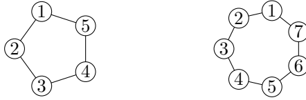
Figure 3.3 – The cycle graphs C_5 , C_7 .
