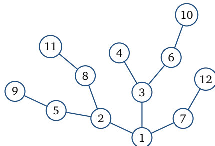
Figure 3.3 – A recursive tree with 12 vertices.
