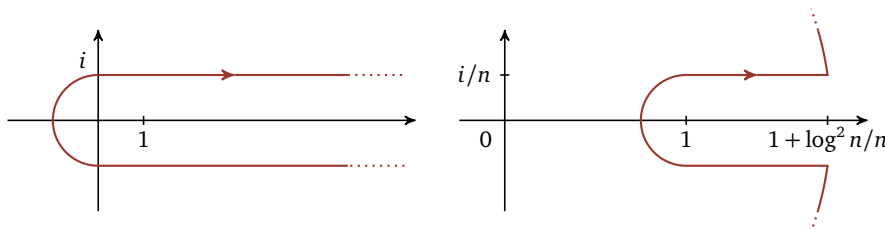
Figure 3.1 – The contours \gamma and \gamma_n .
