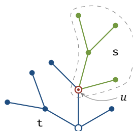
Figure 1.3 – The tree \mathfrak{t} \otimes (u, \mathfrak{s}) .
