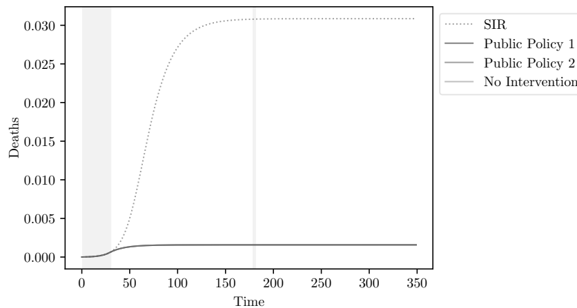
Figure 1.10: Cumulative number of deaths under Public Policy 1 and Public Policy 2.
