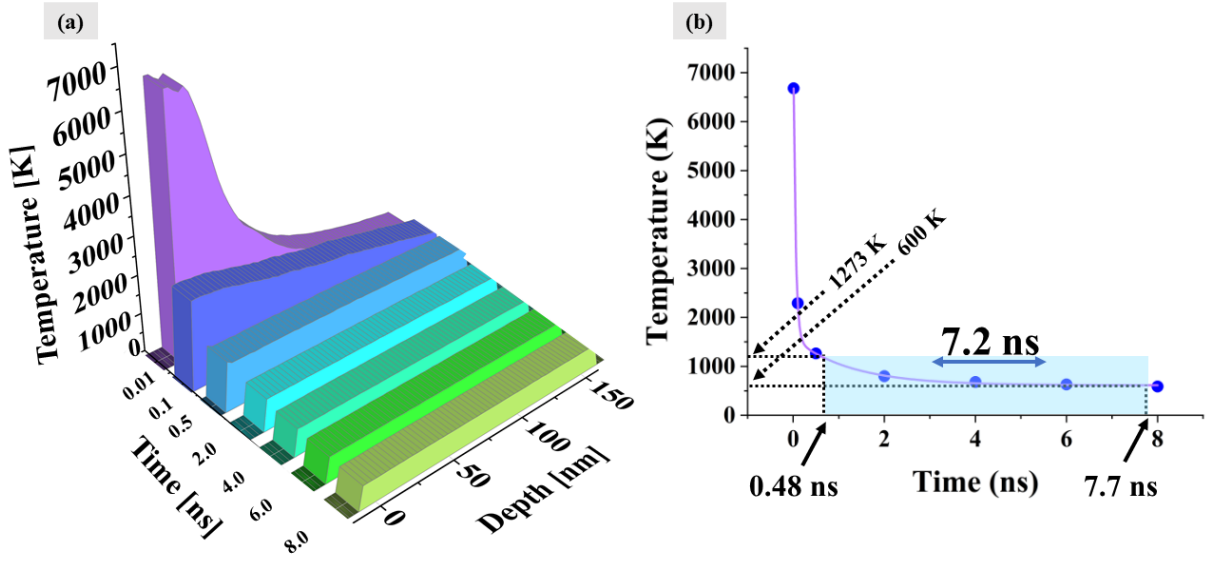
Figure 4.9: (a) Temperature depth profile in W irradiated by femtosecond laser with Fp = 0.32 J/cm 2 and N = 20 at different snapshots of time obtained from TTM-MD simulations (b) Temperature evolution versus time at the surface of the W sample.
