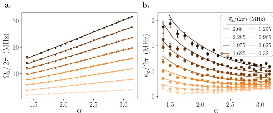
Figure 5.4: a. Dots: Inferred rotation frequency \Omega_Z as a function of cat code frequency \alpha , and for various mean drive amplitudes \bar{\epsilon}_Z/2\pi = 0.32, 0.625, 0.965, 1.295, 1.625, 1.955, 2.285, and 2.66 MHz from bright to dark orange. Lines: expected rotation frequency \Omega_Z = 4\text{Re}(\bar{\epsilon}_Z\alpha) around Z . b. Dots: Inferred decay rate \kappa_Z as a function of |\alpha| for the same drive amplitudes. Lines: simulated decay rate with g_2/2\pi = 6 MHz as a fit parameter and the same detuning \Delta_b as in Fig. 4.14b.
