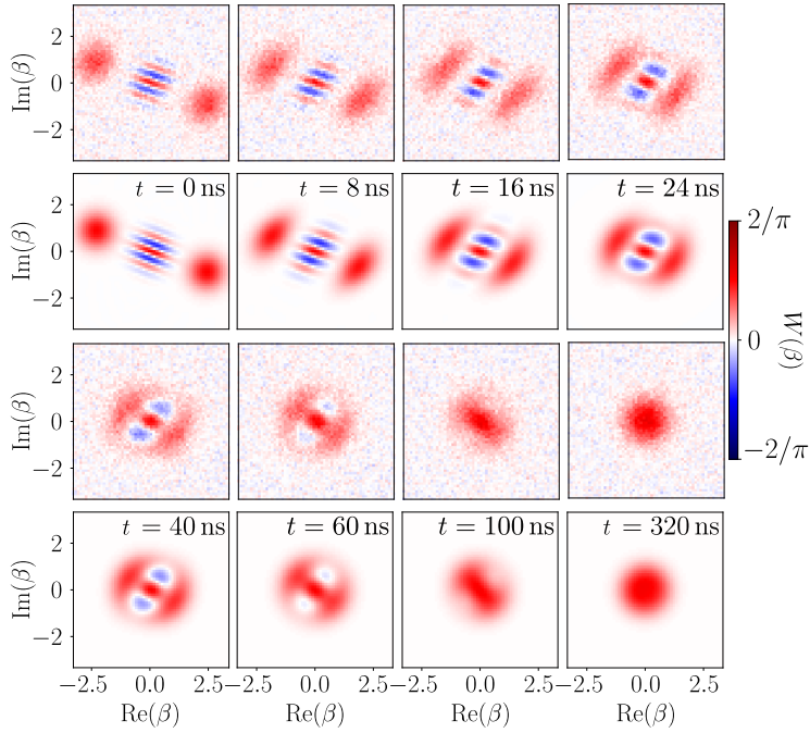
Figure 4.10: Evolution of the Wigner functions of the memory starting close to a cat state |C_{\alpha}^{+}\rangle and under the effect of two-photon dissipation at \phi_{\text{QEC}} without driving the buffer. First and third lines: measured Wigner functions at various times indicated on the figure. Second and fourth lines: simulated Wigner functions of the memory without the adiabatic elimination of the buffer, and assuming a two-photon coupling rate g_2/2\pi = 6 MHz (Fig. 5.4b).
