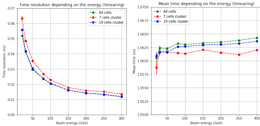
Figure 4.27: Standard deviation (on the left) and mean time (on the right) of the Gaussian fit done on T_0A distributions as a function of the beam energy. In red 7 cells are used, in blue 19 cells, and all the cells in green.
