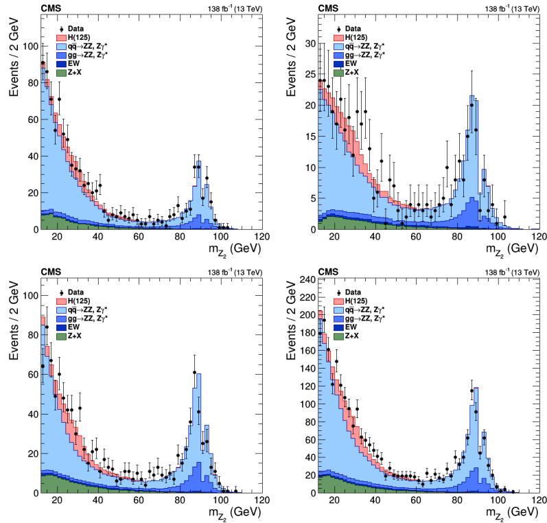
Figure 5.10: Distribution of m_{Z_2} using the full Run-2 statistic. Black points represent data, H signal in pink, and the backgrounds are q\bar{q} \rightarrow ZZ in light blue, gg \rightarrow ZZ in blue, EW in dark blue, and Z + X in green. The plot on top left corresponds to 4\mu , on top right to 4e , on bottom left to 2\mu 2e , and on bottom right to 4l .
