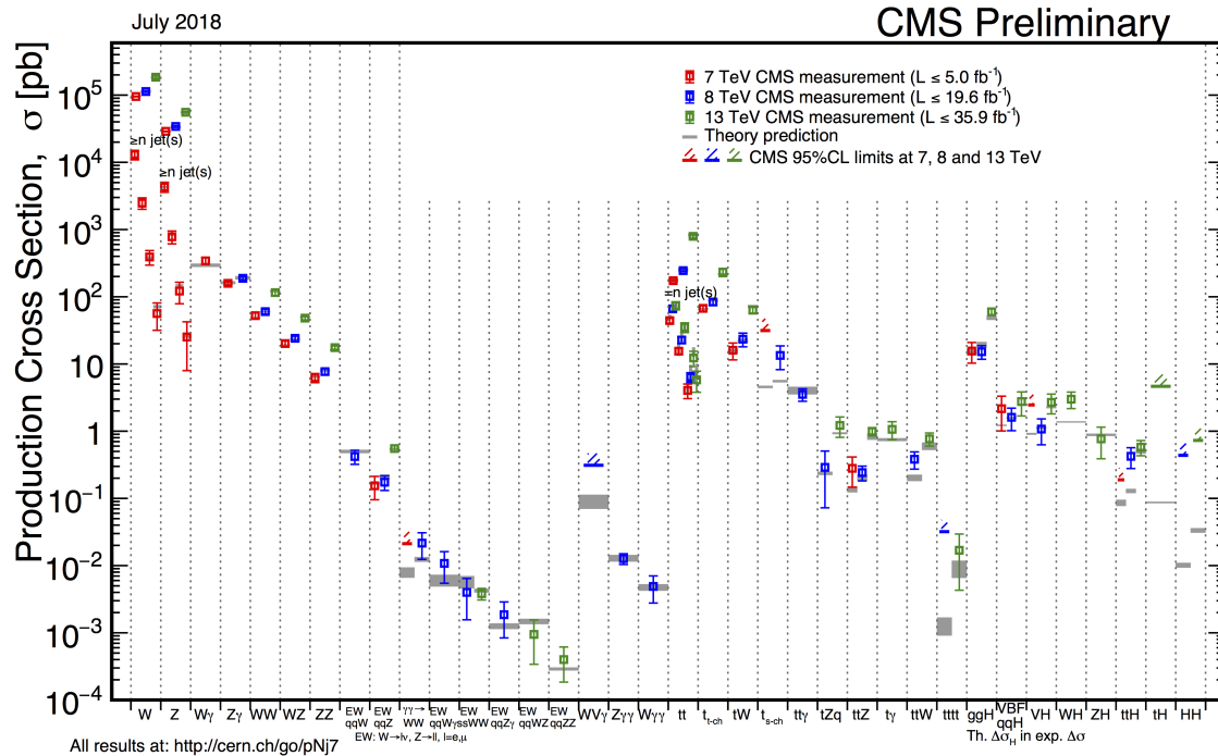
Figure 2.19: Summary of the cross-section measurements of Standard Model processes produced by the CMS experiment. Measurements are done for \sqrt{s} = 7 TeV in red, 8 TeV in blue, and 13 TeV in green.
