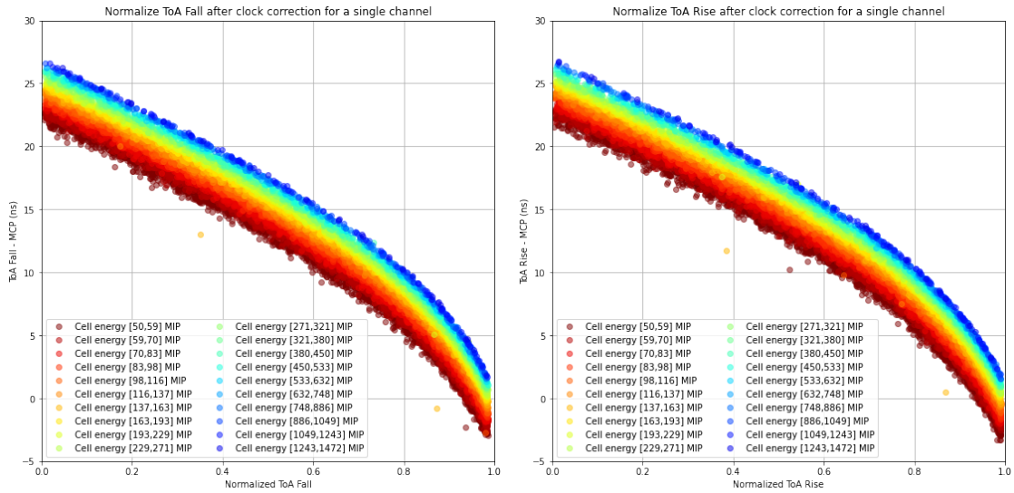
Figure 4.16: TW depending on the normalized ToA . Each colour corresponds to a specific cell energy range. The ToA_{\text{fall}} is on the left, and the ToA_{\text{rise}} is on the right.
