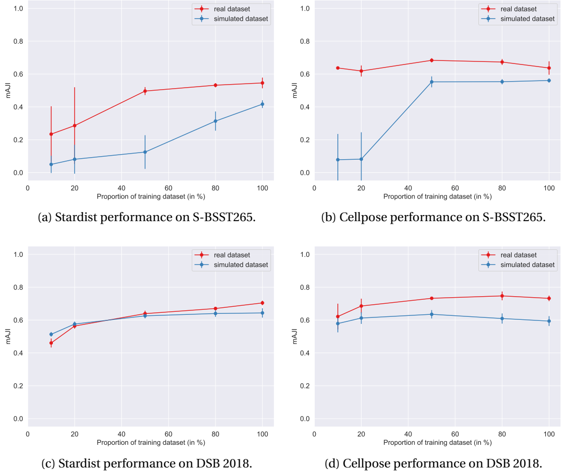
Figure 4.11: A comparison of the evolution of the mAJI score measured on the S-BSST265 and DSB 2018 datasets as a function of the size of the training set. Each point corresponds to the average ( \pm stddev) of the mAJI score measured with only a certain proportion of the available training set. The red lines are derived from a model trained on a dataset consisting only of real images and the blue lines are derived from one consisting only of simulated images.
