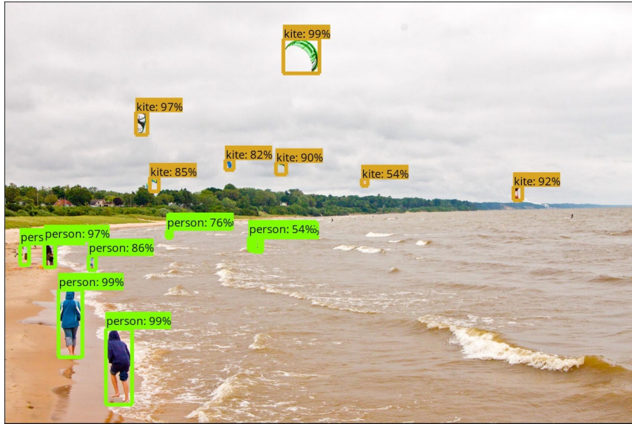
Figure 2.10: Object detection outputs with a model trained in Tensorflow from Huang et al. [2017]. Each result is a bounding box, encompassing an object of class according to a certain confidence score.
