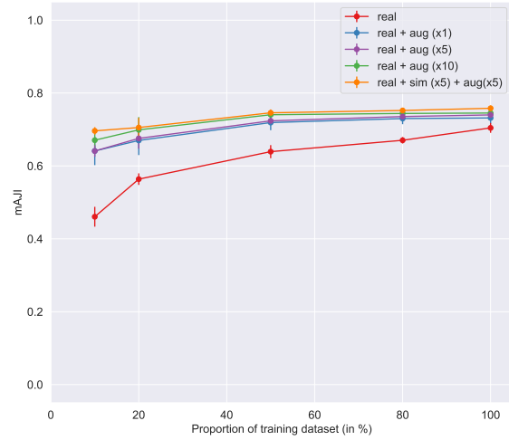
(b) Stardist perf. on DSB 2018, data augmentation.
