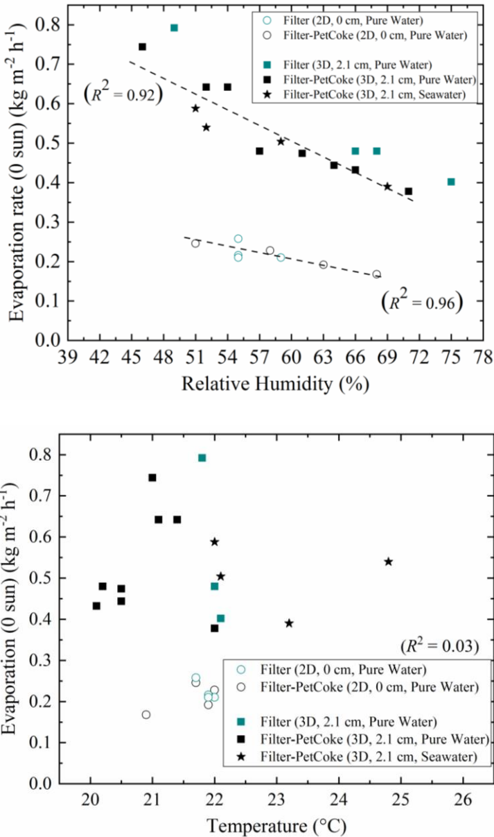
Figure 5.11. Upper; Correlation between the atmospheric relative humidity and the 0 sun evaporation rate, Lower; between the atmospheric temperature and the 0 sun evaporation rate.
