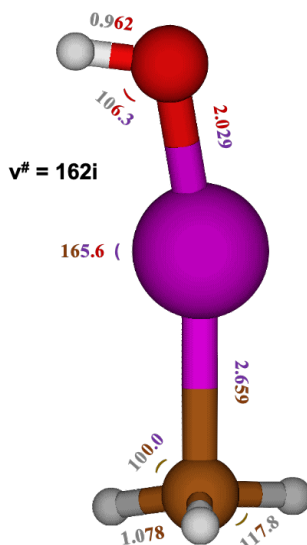
Figure 6.15: Schematic representation of TS 10 without additional H 2 O molecule optimized at the M06-2X/6-311+G(2df,2p) level of theory. The distances are in Angstroms; the angles are in degrees; the imaginary vibrational frequency is in cm -1 .
