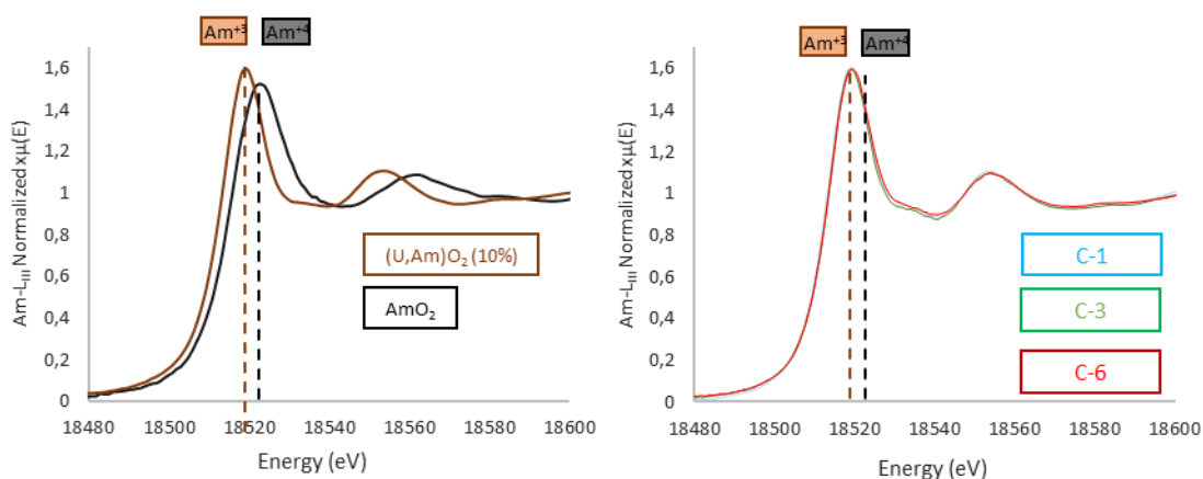
Figure 97 Am-L III XANES Analysis of Capra4 Samples. Left Side: reference spectra for comparison. Right Side: C-1 is 44 days old, C-3 is 134 days old, C-6 is 8000 days old Capra4 samples compared with the reference positions.
