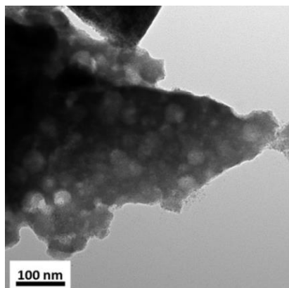
Figure 25 TEM image of AmO 2 showing a high concentration of large He bubbles (white spots) after 36 dpa of damage [10].
