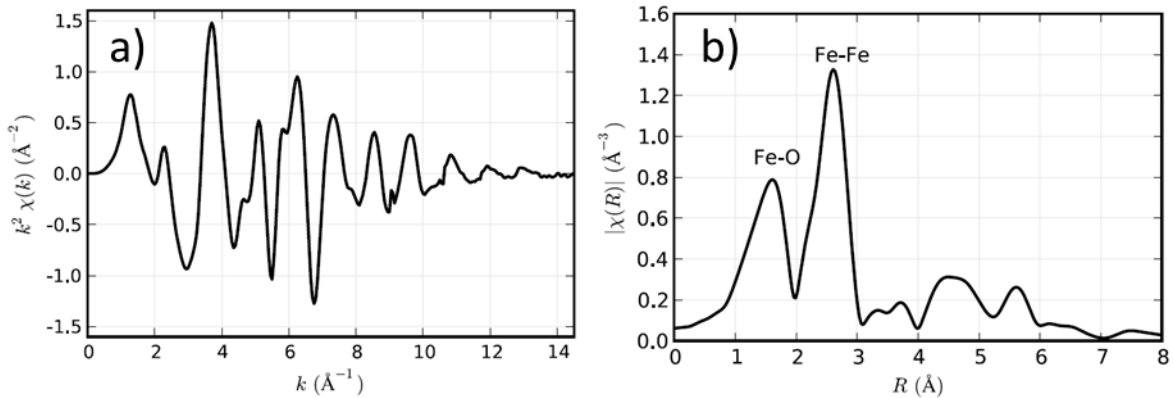
Figure 42 The EXAFS spectrum obtained for the Fe K edge of FeO, with a) k^2 weighting applied to EXAFS spectra b) the Fourier transform of the k -weighted XAFS, revealing the contributions originating from neighboring atoms of both Fe-O and Fe-Fe [134].
