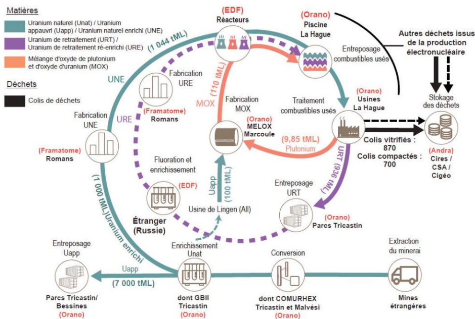
Figure 1 Simplified diagram of a closed fuel cycle adapted for the French nuclear program [2]
