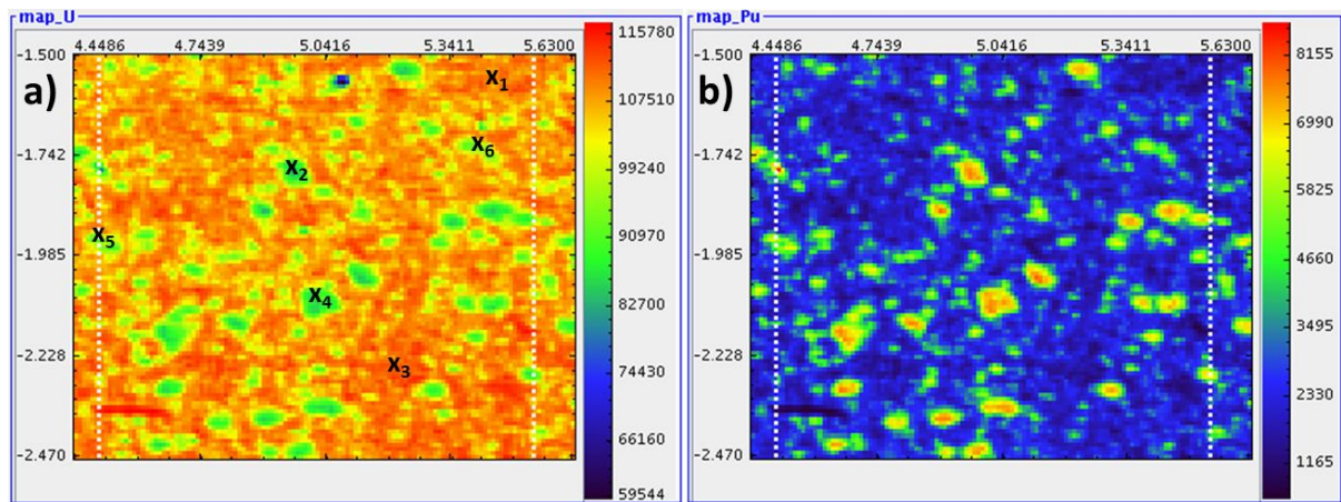
Figure 69 X-ray Fluorescence map of a selected zone in the annealed MIMAS sample, a) Uranium mapping, b) Plutonium mapping. For the mappings, the x- and y- axis are shown in mm scale and the color scale corresponds to the number of counts of the fluorescence emission.
