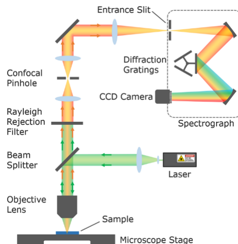
Figure 38 : Typical layout of a Raman microscope with a fiber-coupled laser source and spectrometer (image from Edinburgh instruments)
