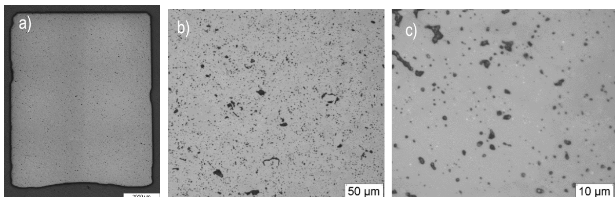
Figure 140 Optical image of the MIMAS sample surface after annealing a) image of the whole pellet (reconstructed from \times 1.25 images), b) and c) at larger magnifications
