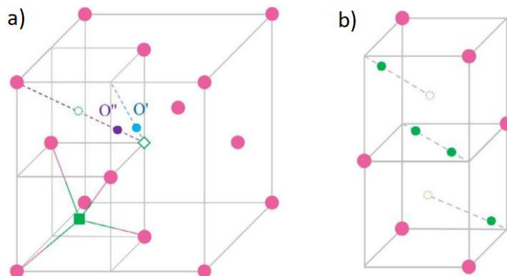
Figure 4 Incorporating additional oxygen atoms at the \text{UO}_2 structure. a) Positions of the \text{O}' and \text{O}'' atoms and formation of oxygen vacancy b) The (2:2:2) Willis cluster model (Pink dots denote normal U atom, green cube denotes normal O atom, green dots denote O interstitial, green open diamond denotes the octahedral site and green open dots denote O vacancies [26].
