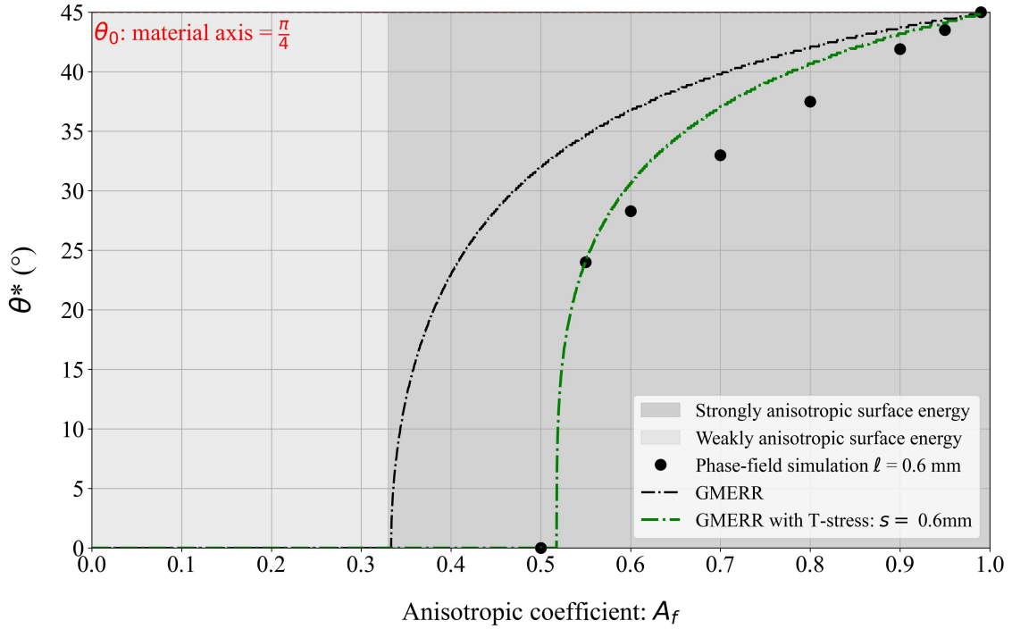
Figure 5.2 Comparison between numerical results with choice of \ell=0.6\text{ mm} and GMERR prediction for short sample at fixed material axis \theta_0=45^\circ with different anisotropic coefficient. The black-dot line represents the GMERR predictions without considering the T -stress, while the green curve represents the predictions that take into account the T -stress effect.
