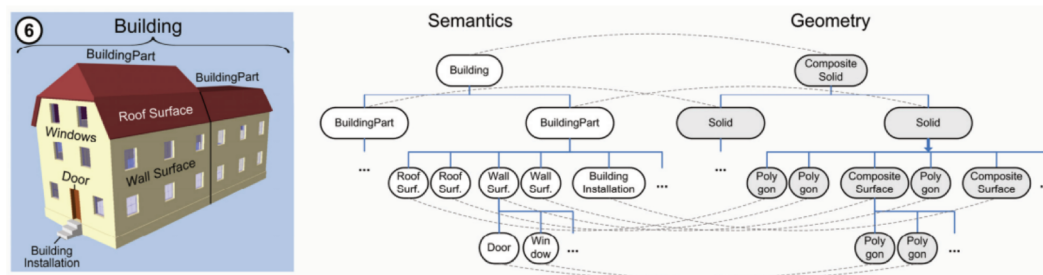
Figure 3.1.: An example of the thematic and geometric classes from CityGML and their relations from Stadler and Kolbe [SK07].
