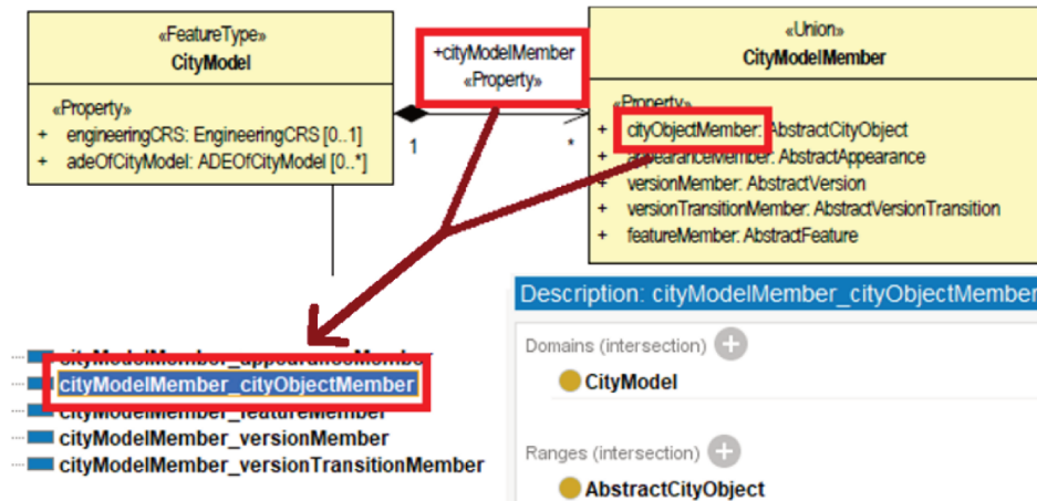
Figure 5.4.: An example of Union flattening (mapping 3) of core:cityModelMember and core:cityObjectMember (top) and their mappings to OWL (bottom) from the CityGML 3.0 UML model.
