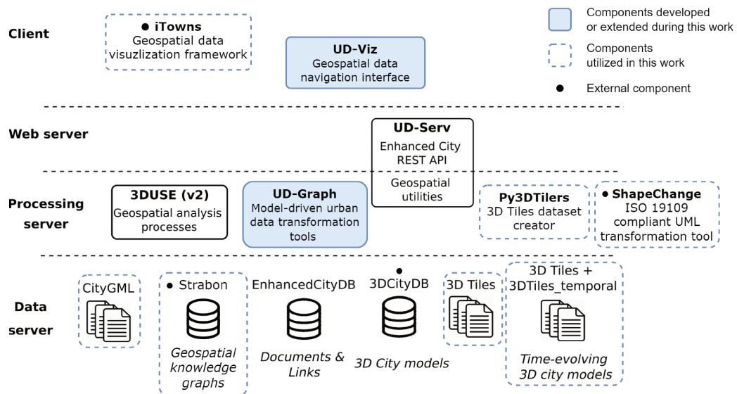
Figure 6.1.: Current software and 4-tier technical architecture of the UD-SV platform extended from [Sam+23]. Components developed or extended during this these are highlighted in blue. Other components or software used during this thesis are encircled in blue.
