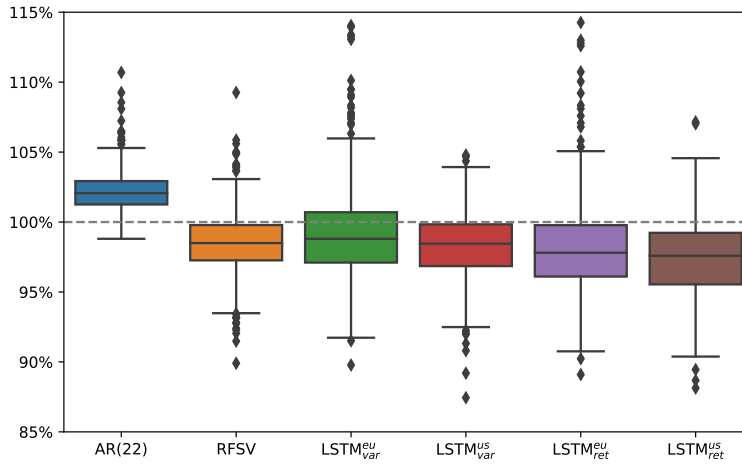
Figure I.9: Boxplot showing models' out-of-sample performances relative to the HAR model for the stocks of the European market. Note that LSTM EU and LSTM US are trained on stocks of the European and US markets respectively.
