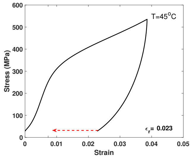
Figure 3.7: Stress-strain diagram at A_f + 5^{\circ}\text{C} obtained from the sample subjected to 2 h of homogenization and then 1 h of aging at 350^{\circ}\text{C} . The residual strain at the end of unloading is presented inside the figure. Arrow represents the strain recovery by re-heating the sample until 100^{\circ}\text{C} and then cooling to room temperature.
