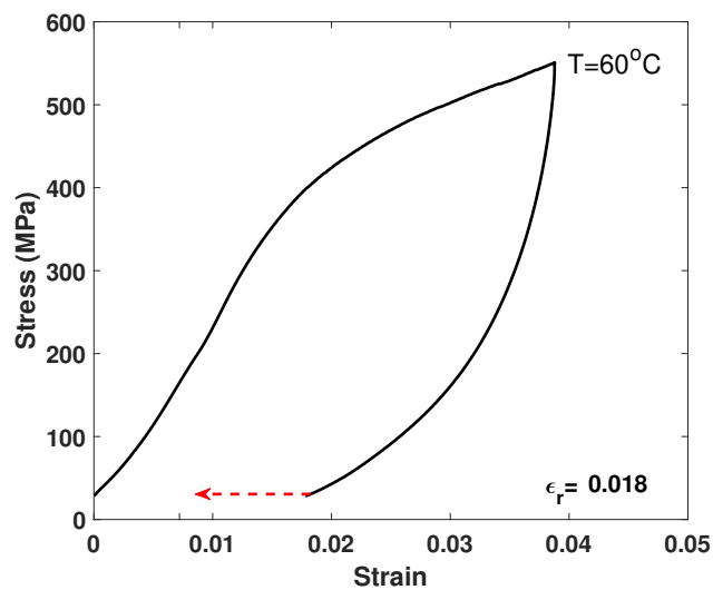
Figure 3.8: Stress-strain diagram at A_f + 5^{\circ}\text{C} obtained from the sample subjected to 5 h of homogenization and then 24 h of aging at 350^{\circ}\text{C} . The residual strain at the end of unloading is presented inside the figure. Arrow represents the strain recovery by re-heating the sample until 100^{\circ}\text{C} and then cooling to room temperature.
