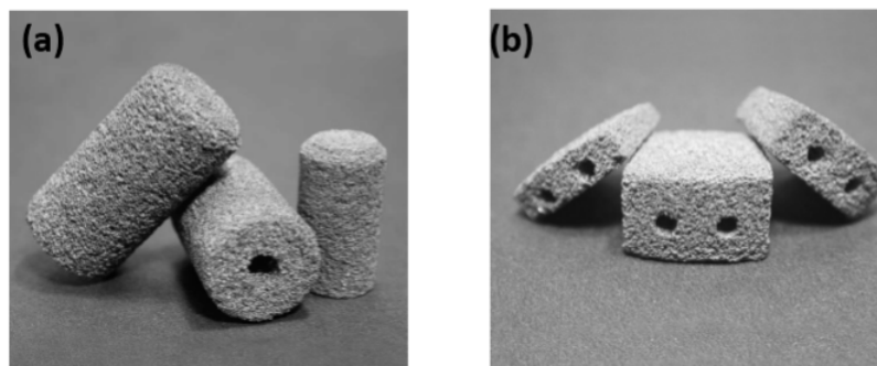
Figure 1.1: a) Cervical spine and b) lumbar spine implants made of porous NiTi [1].
