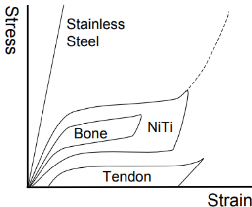
Figure 1.2: Stress-strain curves of stainless steel, NiTi, bone and tendon [1].
