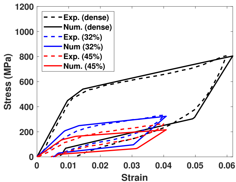
Figure 4.11: Pseudoelastic loops of the NiTi in [8] for different porosity.
