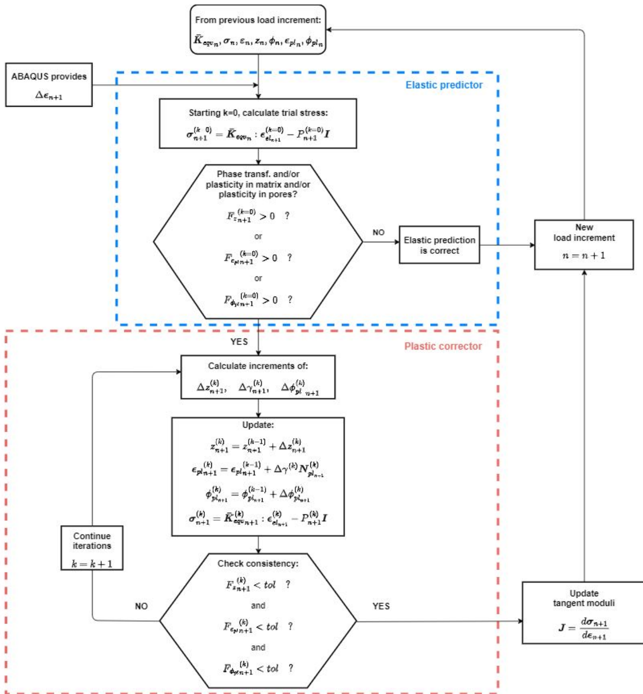
Figure 4.3: Return mapping algorithm for UMAT used in porous SMA modeling.
