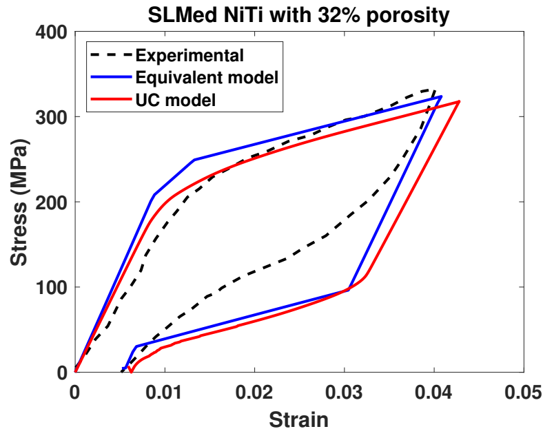
Figure 5.5: Simulation of the uni-axial stress-strain curve of 32% porous NiTi sample in [8] using UC model.
