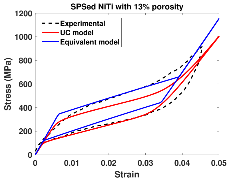
Figure 5.3: Simulation of the uni-axial stress-strain curve of 13% porous NiTi sample in [7] using UC model.
