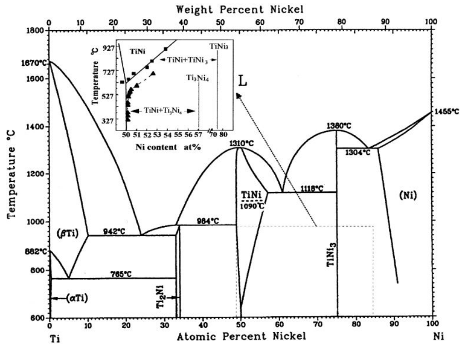
Figure 2.4: Phase diagram of Ni-Ti alloy [5].
