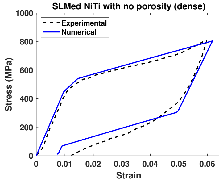
Figure 4.7: Simulation of the uni-axial stress-strain curve of the dense NiTi sample in [8] using phenomenological model.
