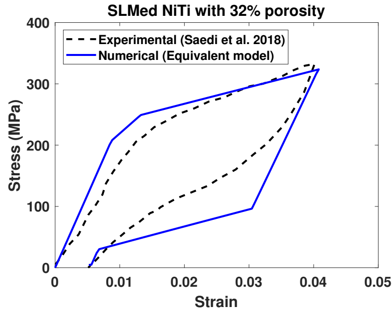
Figure 4.8: Simulation of the uni-axial stress-strain curve of 32% porous NiTi sample in [8] using the effective phenomenological model.
