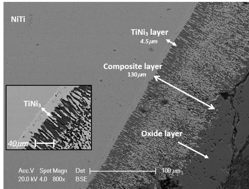
Figure 2.16: Cross-section of the sample subjected to 5 h of homogenization and 24 h aging at 350^\circ\text{C} . Image taken from SEM.
