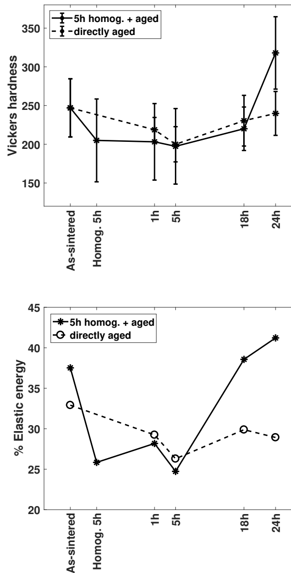
Figure 3.4: Vickers hardness and percentage of recoverable energy after aging at 350°C for different duration. Error bars represent the standard deviations in 10 measurements.
