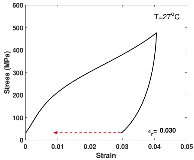
Figure 3.10: Stress-strain diagram at room temperature obtained from the sample subjected to 2 h of homogenization and then 1 h of aging at 350°C. The residual strain at the end of unloading is presented inside the figure. Arrow represents the strain recovery by re-heating the sample until 100°C and then cooling to room temperature.
