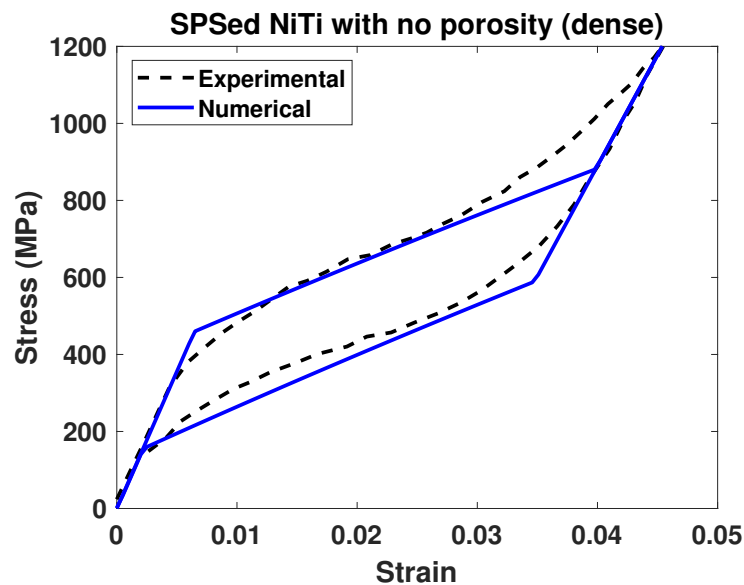
Figure 4.4: Simulation of the uni-axial stress-strain curve of the dense NiTi sample in [7] using phenomenological model.
