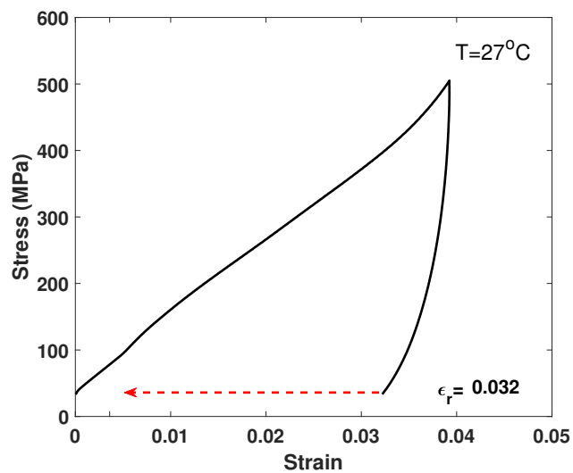
Figure 3.11: Stress-strain diagram at room temperature obtained from the sample subjected to 5 h of homogenization and then 24 h of aging at 350°C. The residual strain at the end of unloading is presented inside the figure. Arrow represents the strain recovery by re-heating the sample until 100°C and then cooling to room temperature.
