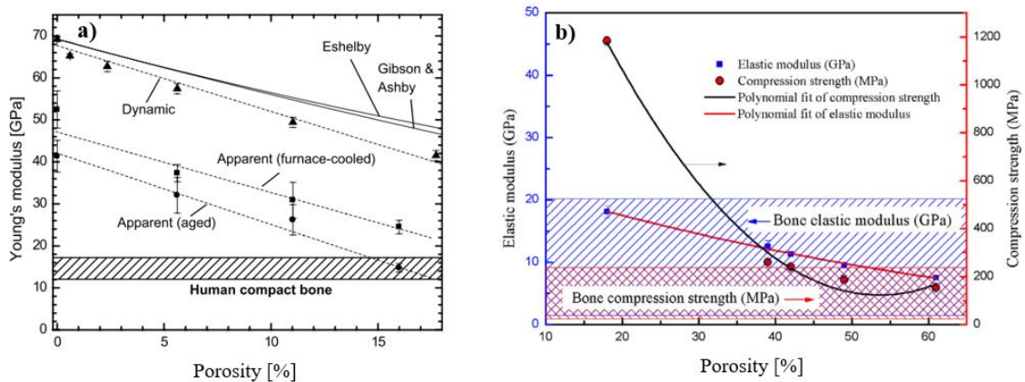
Figure 1.5: Effect of porosity on the elastic modulus and the compressive strength of NiTi alloys studied by a) Greiner et al. [3] and b) Zhang et al. [4].
