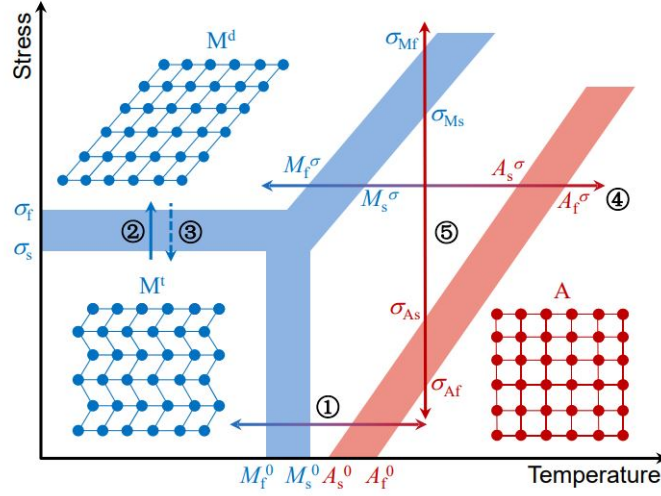
Figure 1.3: Schematic diagram of phase transformation [2].
