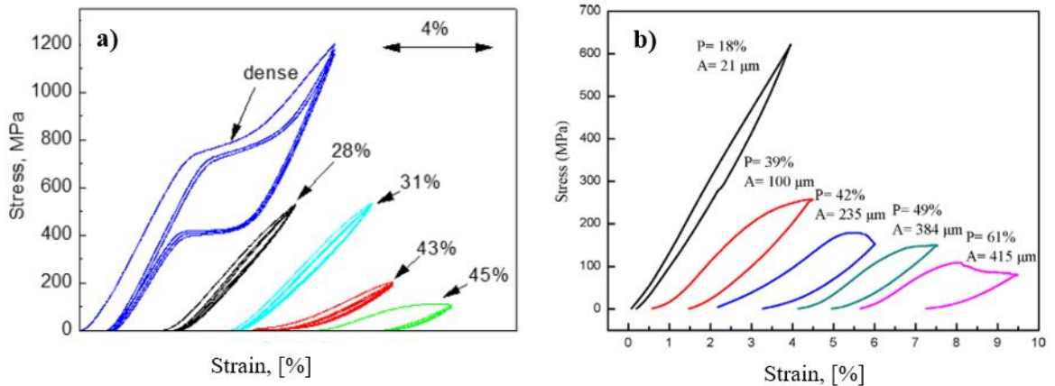
Figure 1.6: Uni-axial compression of NiTi alloys obtained by a) Yuan et al. [1], b) Zhang et al. [4].
