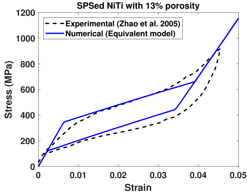
Figure 4.5: Simulation of the uni-axial stress-strain curve of 13% porous NiTi sample in [7] using the effective phenomenological model.
