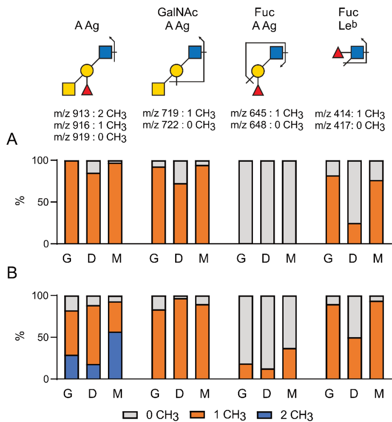
Figure 9. Relative quantification of native and methylated form of A Ag and Leb Ag. Deuteromethylated N -glycans of C. gigas and O. edulis were analyzed by LC-MS 2 . Characteristics MS 2 ions for individual antigens and their respective methylated forms were identified as depicted on top. Proportions of methylated individual glycan epitopes were quantified in N -glycans isolated from the three tissues of (A) C. gigas and (B) O. edulis . Light gray, 0 CH 3 group; orange, 1 CH 3 group; blue, 2 CH 3 groups. G, gills; D, digestive tract; M, mantle.
