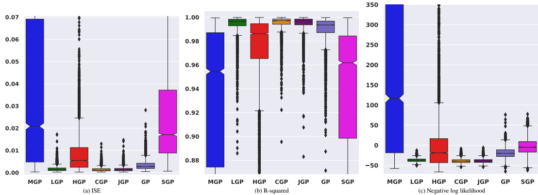
Figure A.2: Box-plots of the results of different Gaussian process models in predicting the true function g(t) = \sum_{j=1}^P c_j \varphi_j(t) , where c_j generated independently from \mathcal{N}(0, \lambda_j) . Where MGP: Matérn, LGP: Legendre, HGP: Hermite, CGP: Chebyshev, GP: standard GP, SGP: Sparse GP.
