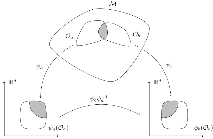
Figure II.2: Two charts and their transition maps.
