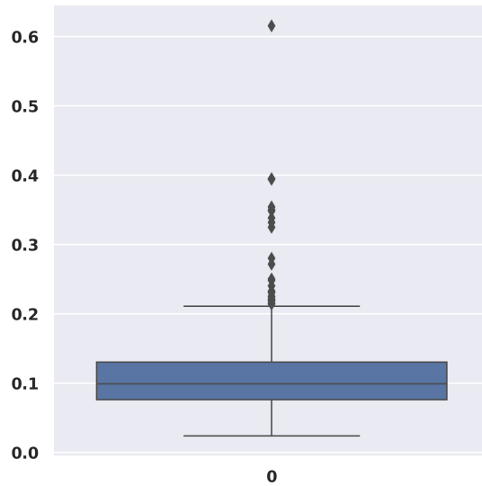
Figure V.1: The boxplot of geodesic distance error of the reconstruction and the true of P_L .
