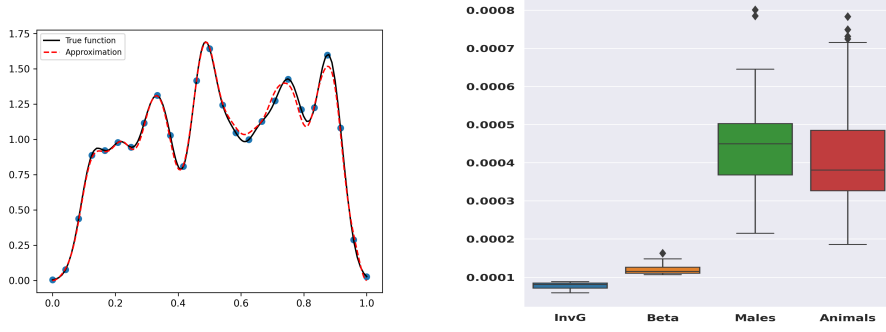
Figure IV.8: Left: The true PDF (black), the training points (blue) and the NN-based approximate (red). Right: The boxplots summarizing ISE for NN-based method on 4 dataset.
