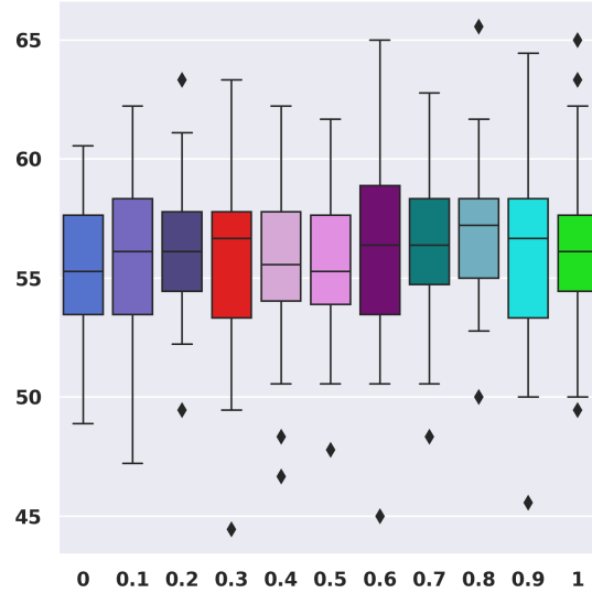
Figure V.9: The Box-plot of accuracy of the combined model for datasets of histograms from images of cats and dogs.
