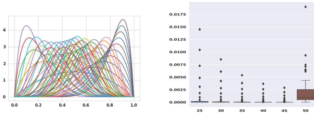
Figure IV.1: Some illustrations of the true functions f_M^2 (left) and the Boxplots of Integrated Square Error (ISE) between the true functions f_M^2 and their approximations \hat{f}_M^2 with different truncation orders: M = 25, 30, \dots, 50 (right).
