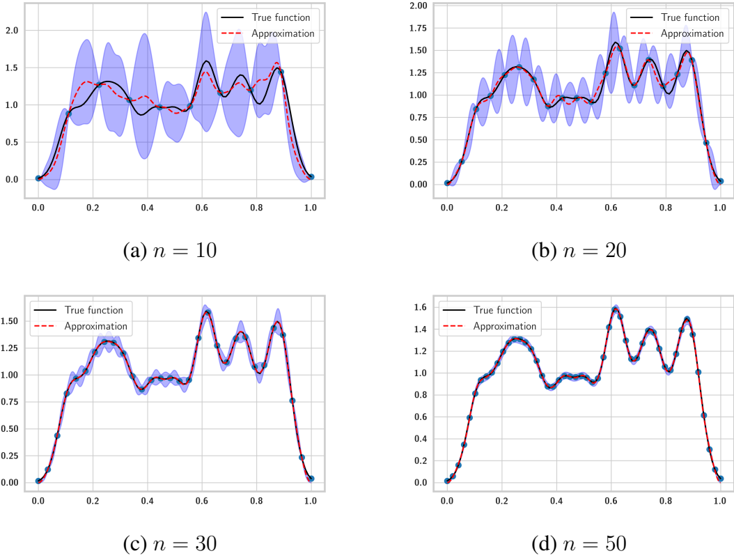
Figure IV.4: The true PDF (black) and observations used for training (blue). The approximated PDF at some unobserved points (red) and the confidence region (cyan) with different data sizes n = 10, 20, \dots, 50 .
