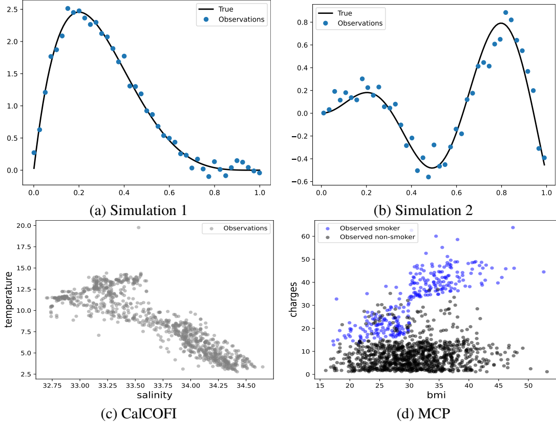
Figure III.2: Some observations from different datasets.
