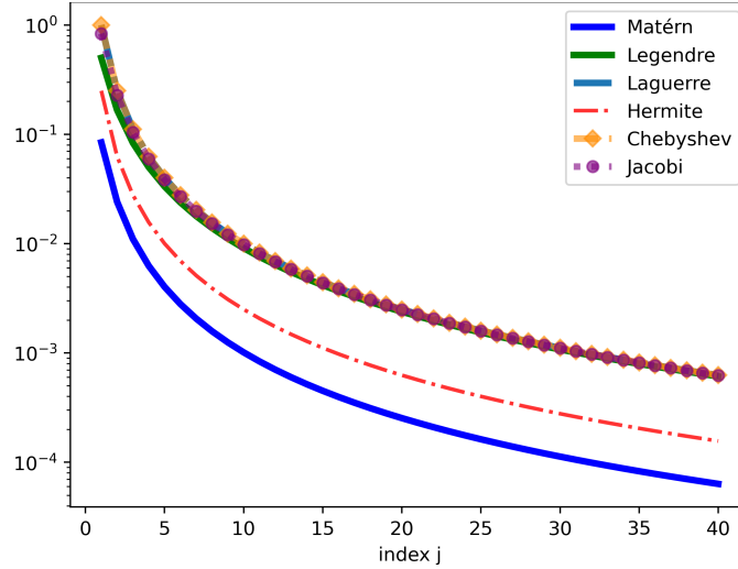
Figure III.1: The eigenvalues \lambda_j of different operators. Where we let: \varepsilon = 2 , \alpha = 1 for Matérn, and \alpha = -0.5 , \beta = -0.3 for Jacobi.
