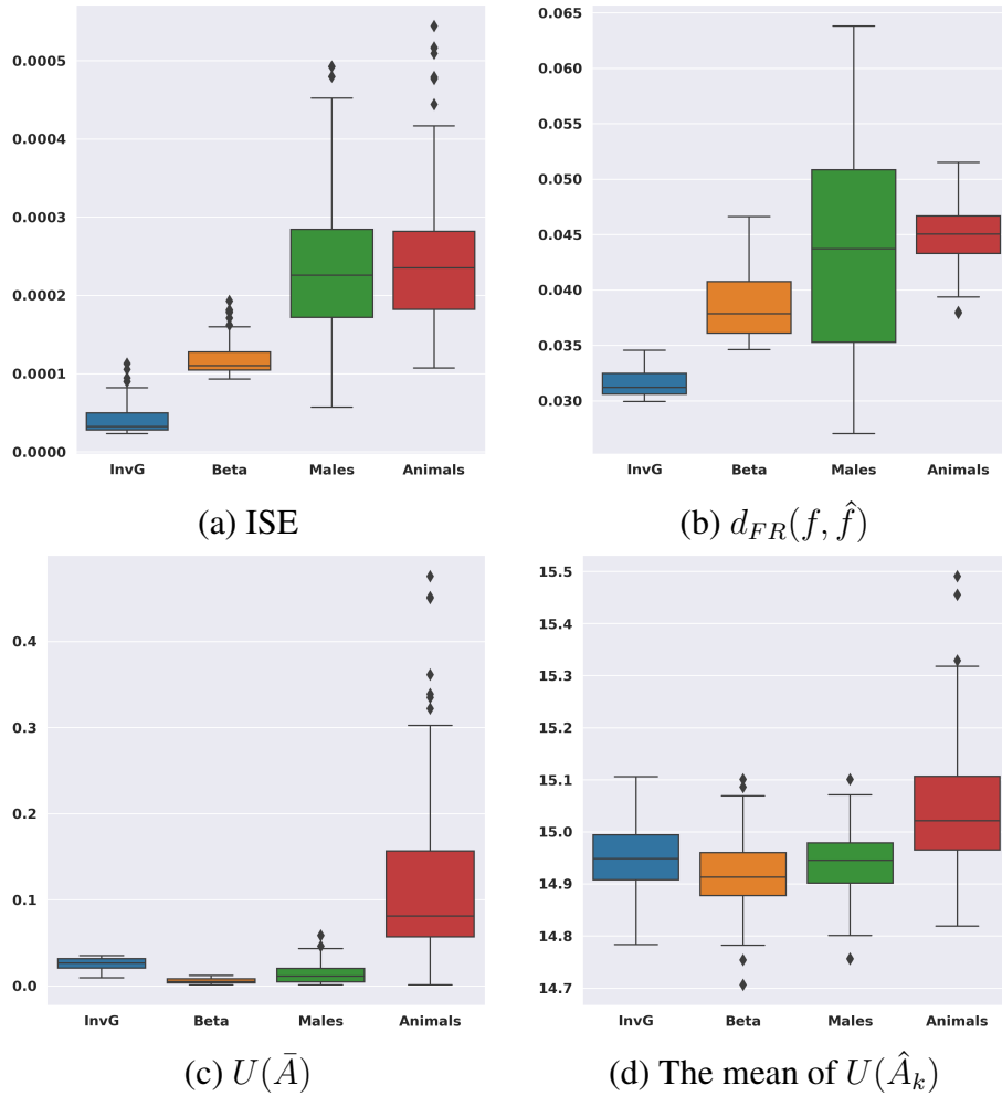
Figure IV.7: Results of cGP using different metrics and various dataset.
