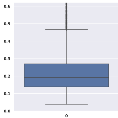
Figure V.6: The boxplot displays the geodesic distance errors on the large dataset of cat image histograms.
