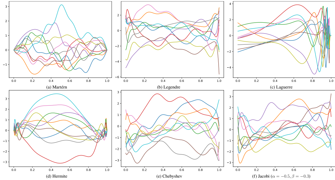
Figure A.1: Realizations of different models.
