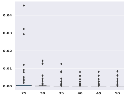
Figure IV.3: The Boxplot of ISE between f_M and \hat{f}_M when n = 25, 30, \dots, 50 and M = 30 .
