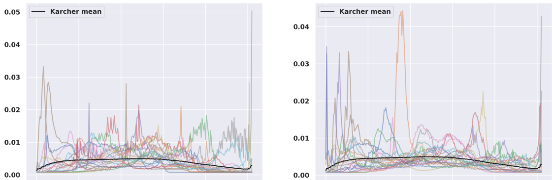
Figure V.5: The images of Karcher mean and some histograms of the large dataset (right) and small dataset (left).
