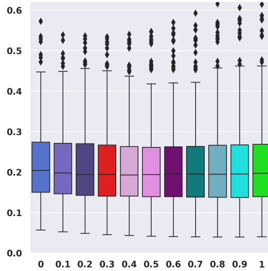
Figure V.7: The boxplots show the reconstruction error for \rho \in \{0, 0.1, 0.2, \dots, 1\} for small dataset of cat image histograms.
