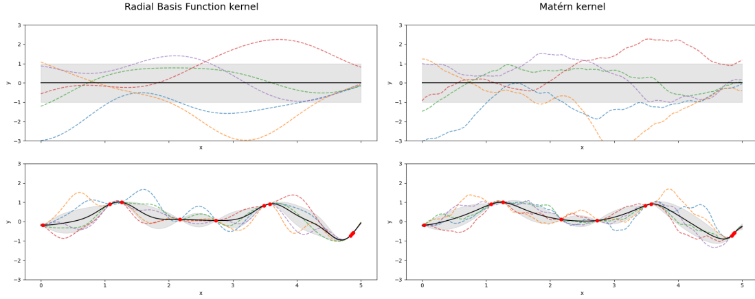
Figure II.1: The prior realizations of Gaussian processes (first row) and the posterior realizations. The black line is the graph of the predictive function in black line, the grey region is the \pm standard deviation, the red points are the observations.
