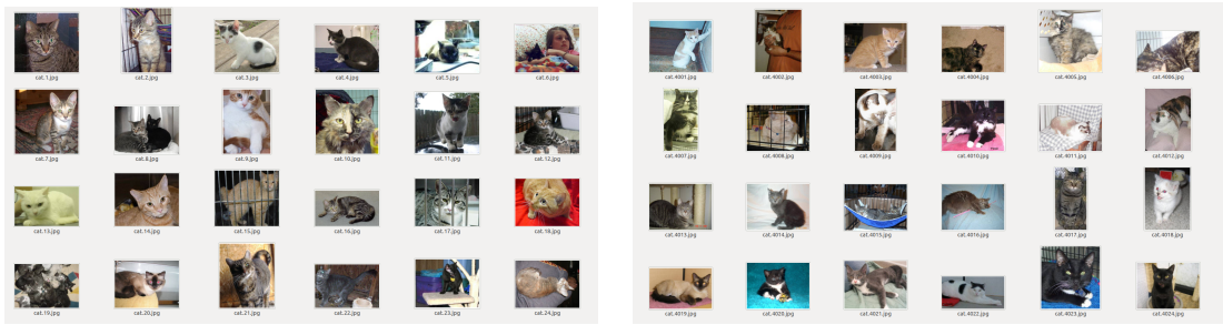
Figure V.4: The images of cats in the large dataset (on the right) and the small dataset (on the left).
