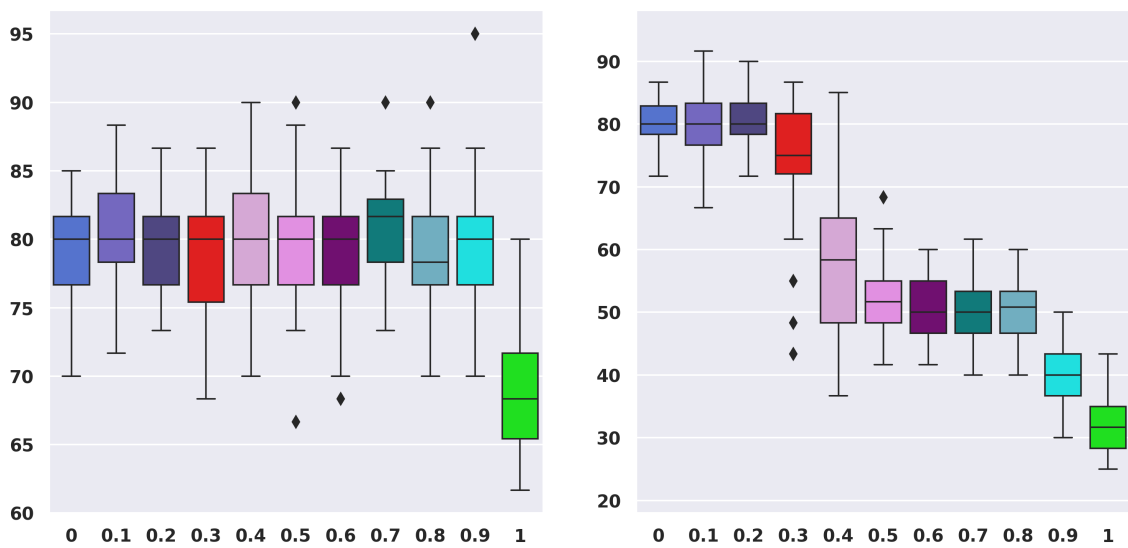
Figure V.8: The Box-plot of the accuracy of the combined models (Left column): the large dataset is Human, (Right column): the large dataset is Heart beats.
