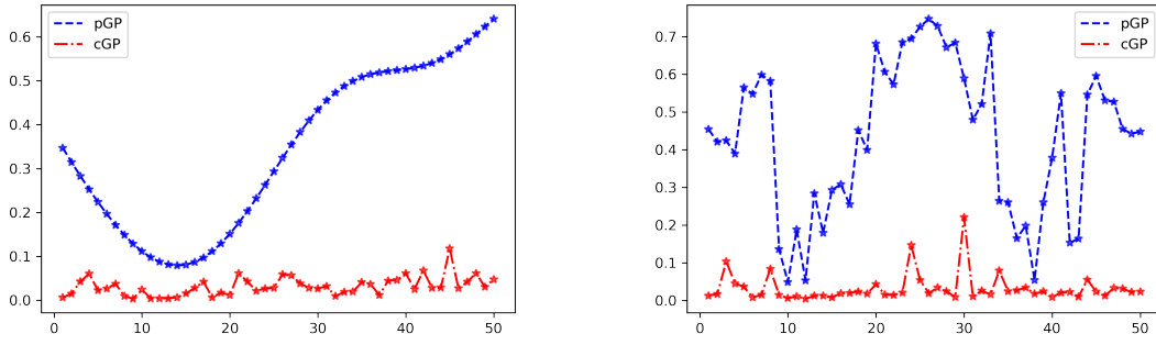
Figure IV.6: Comparison between pGP and cGP: The ISE for several PDFs between 1 and 50 along a geodesic arc as an increasing variation of distance (left) and along a circle as an increasing variation of the angle at a fixed radius (right).
