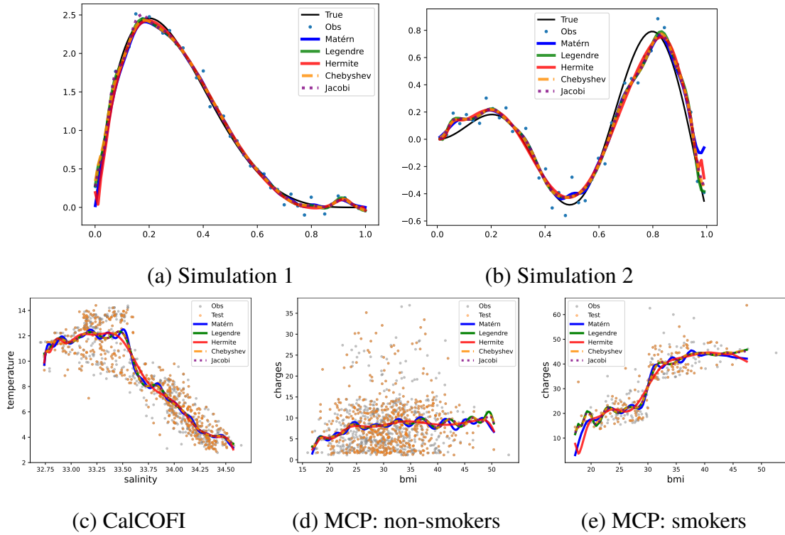
Figure III.3: Illustration of the prediction results with LCGP.
