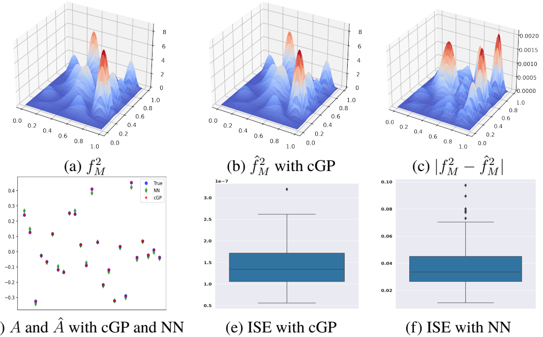
Figure IV.9: Top: An example of a true PDF (a), its approximate with cGP (b) and the difference between them (c). Bottom: The true coefficients in blue and the estimated coefficients in red (d), the boxplot summarizing the \text{ISE}(f_n, \hat{f}_n) from cGP (e) and the NN (f).
