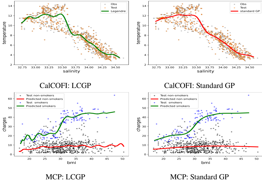
Figure III.4: The prediction results of the proposed method (left) versus comparative methods (right).
