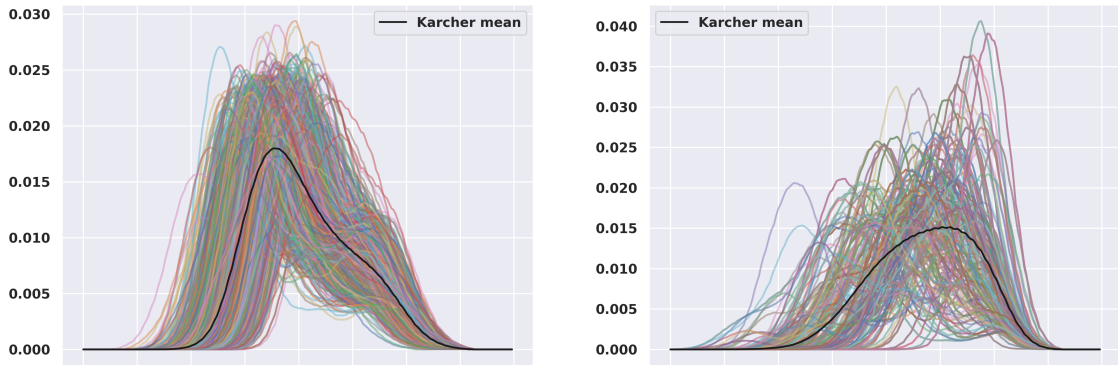
Figure V.2: The data and the Karcher mean of (Left): P_L , (Right): P_S .
