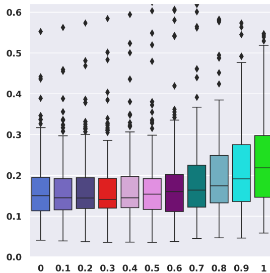
Figure V.3: The boxplots of the reconstruction error for \rho \in \{0, 0.1, 0.2, \dots, 1\} .
